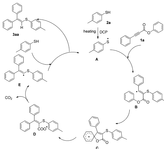
Scheme 6. Proposal Mechanism
