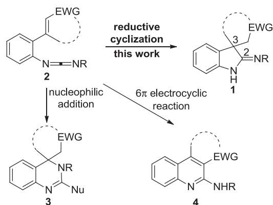
Scheme 1. Synthetic strategy.
