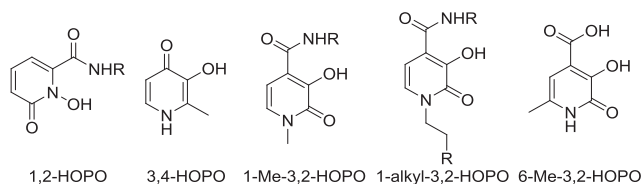
Figure 1. Examples of the hydroxypyridinone family.
