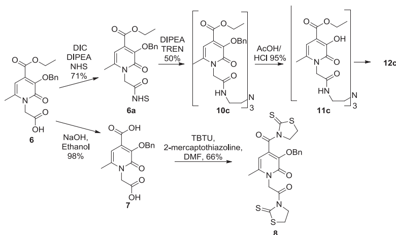
Scheme 4. Reactivity of functionalized 6-Me-3,2-HOPO.
