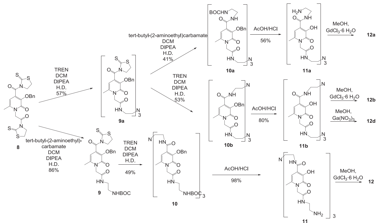
Scheme 5. Synthesis of hexadentate HOPO-based ligands 11–11b .
