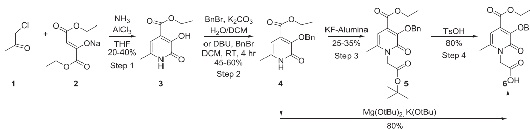
Scheme 1. Synthesis of bifunctionalized 6-methyl-3,2-HOPOs, 5 and 6 .
