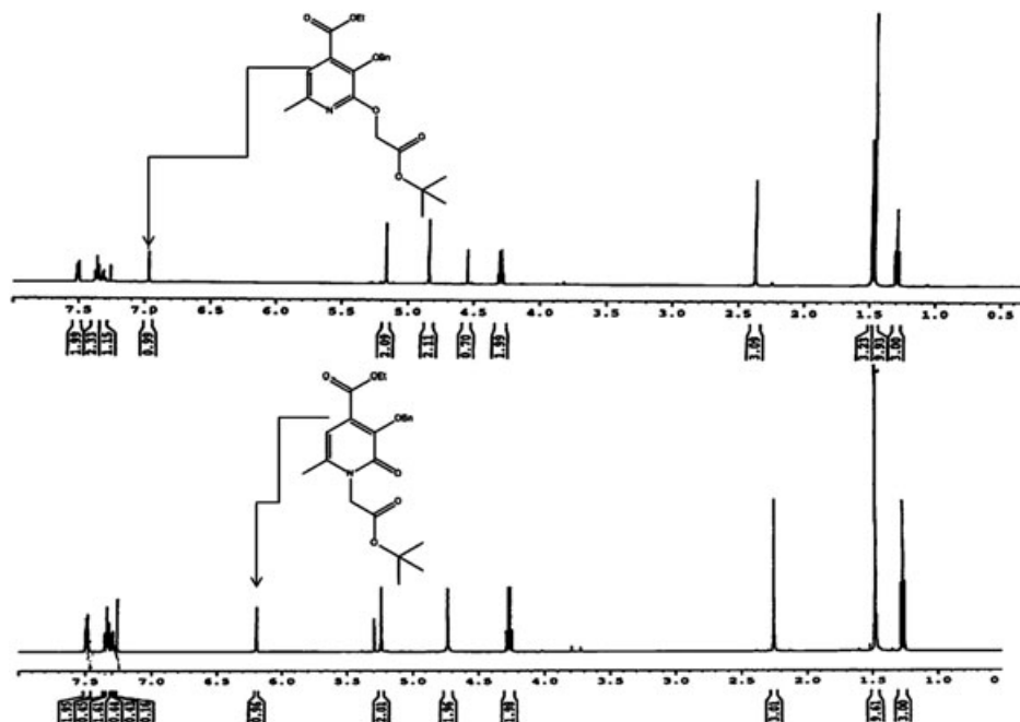
Figure 2. ^1\text{H} NMR comparison between resulting products of competitive N -5 (bottom) versus O -alkylation 5a (top).
