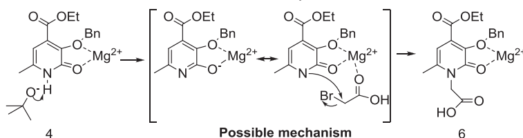
Scheme 3. Possible mechanism of N -alkylation of 6-Me-3,2-HOPO 4 .
