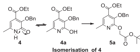
Scheme 2. O -Alkylation of the enolate form of 6-Me-3,2-HOPO 4 .
