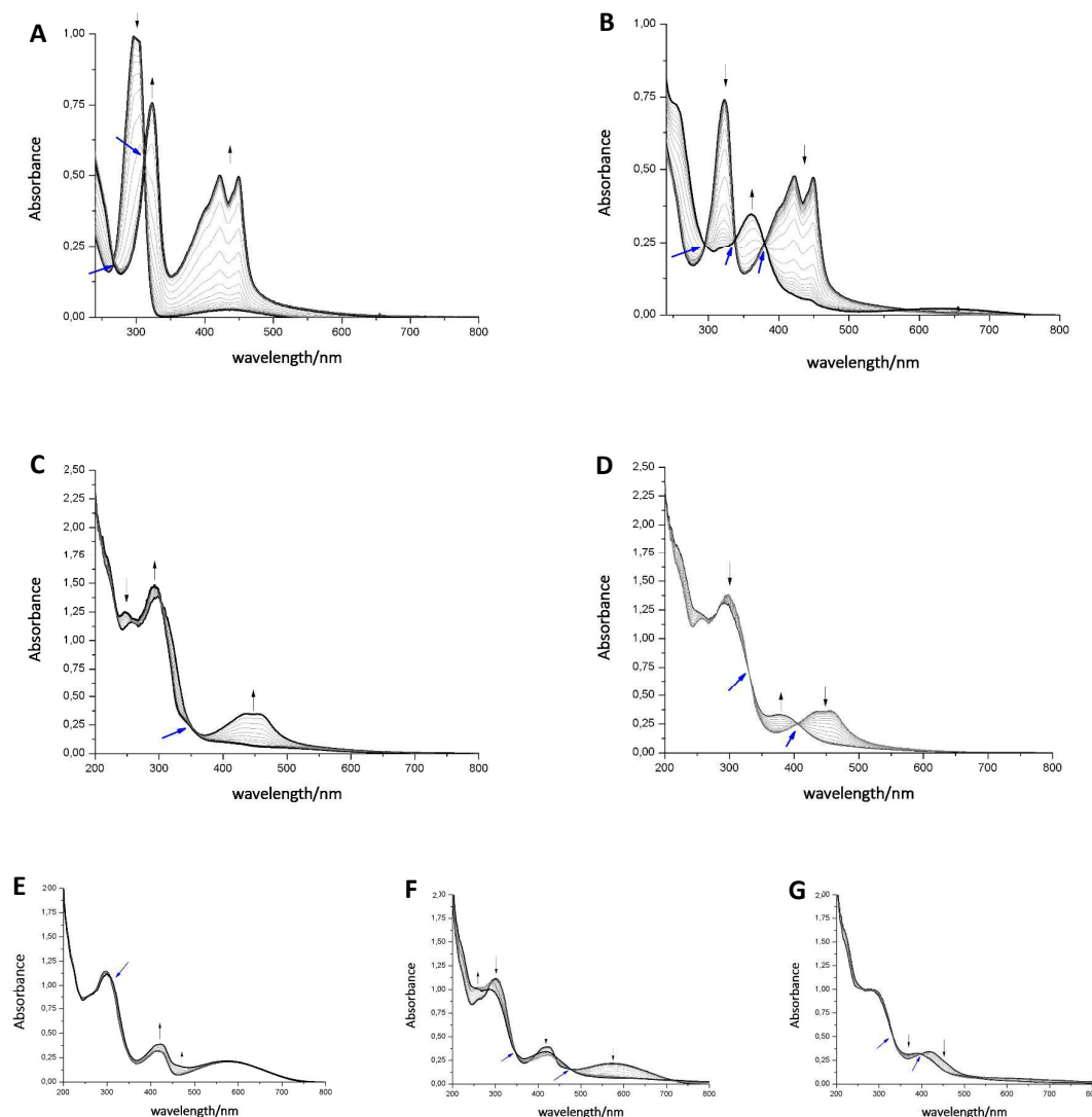
Figure 4: Spectroelectrochemical studies of compounds 9b (A: first peak, B: second peak), 1b o (C: first peak, D: second peak) and 1b c (E: first peak, F: second peak, G: third peak). One spectra-set collaterates with one cathodic wave. Black arrows indicate increase/decrease of maxima; blue arrows assign isosbestic points.
