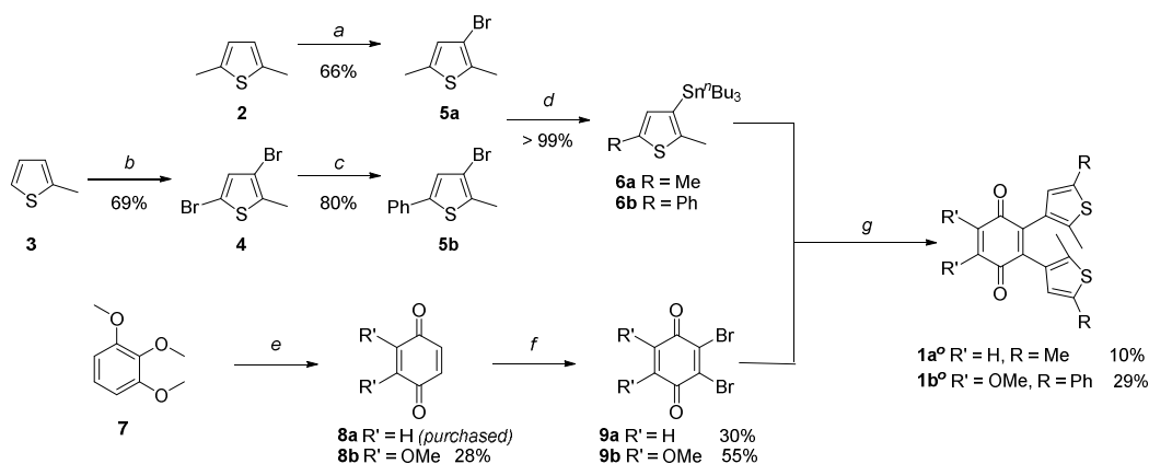
Scheme 1: Synthesis of photochromic Coenzyme Q mimetics 1a o and 1b o : a : NBS, AcOH, 2h, 66%. b : Br 2 , AcOH, 18h, r.t., 69%. c : PhB(OH) 2 , Pd(PPh 3 ) 2 Cl 2 , AsPh 3 , Na 2 CO 3 (2M, aq), THF, 16h, 80 °C, 80%. d : sec BuLi, SnBu 3 Cl, dry THF, -78 °C to r.t., quantitative. e : K 3 [Fe(CN) 6 ], H 2 O 2 , AcOH, r.t., 28%. f : Br 2 , H 2 SO 4 , Et 2 O, 1h; then Ag 2 O, Et 2 O, 1h, 30% for 9a ; 55% for 9b . g : Pd(PPh 3 ) 4 , CuI, dry toluene, 85 °C ( 1a o ) or 115 °C ( 1b o ), 16h, 10% ( 1a o ) or 29% ( 1b o ).
