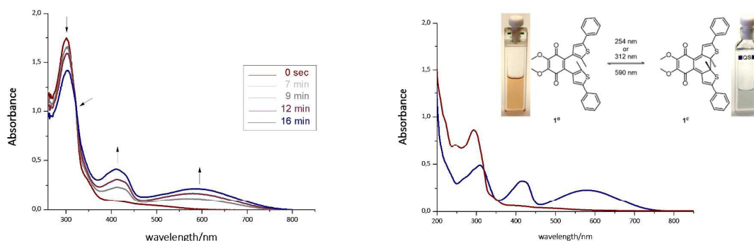
Figure 2: Left: Photoisomerization of 1b° in DMSO (30 μM, irradiation with 312 nm). Right: Spectra of isolated photoisomers 1b° (red line, maxima at 247 nm and 297 nm) and 1b^c (blue line, maxima at 307 nm, 415 nm and 583 nm) in MeCN (isosbestic point at 317 nm). For further details see Supporting Information.
