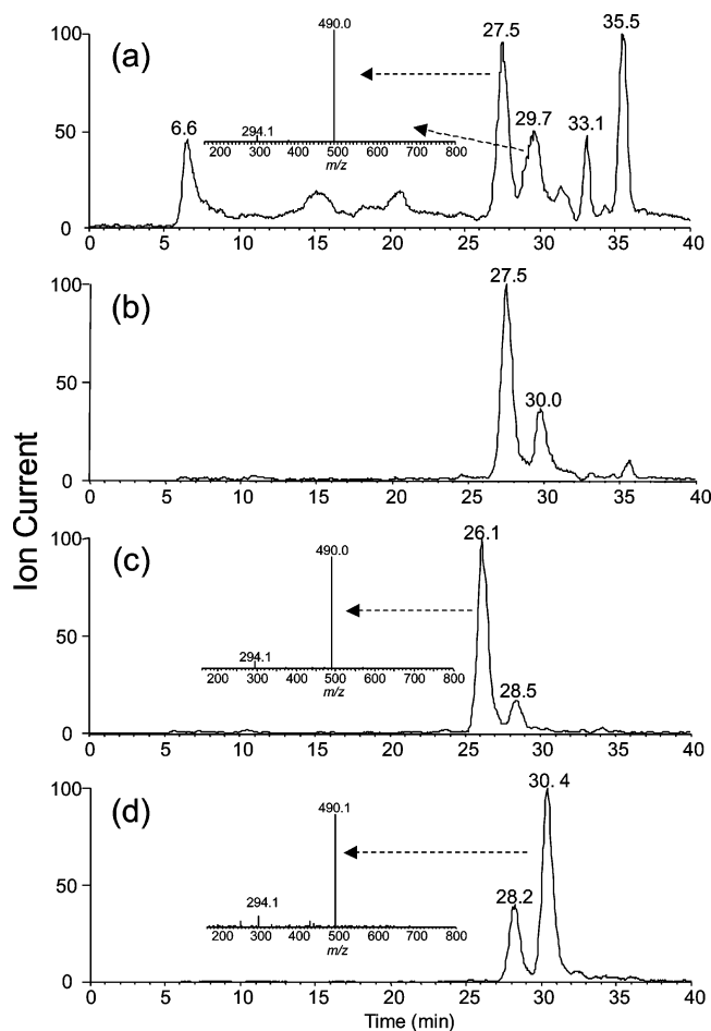
Figure 5. LC-MS/MS of the \gamma -irradiation mixture of d(GT) under anaerobic condition. The mass spectrometer was set to monitor the fragmentation of the ion of m/z 588 in the positive-ion mode: (a) Total ion chromatogram for the fragmentation of the m/z 588 ion with the injection of 4-nmol \gamma -irradiation mixture of d(GT). (b) Selected-ion chromatogram for the m/z 588 \rightarrow m/z 490 transition for the same LC-MS/MS analysis as in (a). (c) Selected-ion chromatogram for the m/z 588 \rightarrow m/z 490 transition with the co-injection of the 1.3-nmol \gamma -irradiation mixture of d(GT) and 5 pmol of the XL lesion initiated from d(GT 1 *). (d) Selected-ion chromatogram for the m/z 588 \rightarrow m/z 490 transition with the co-injection of the 0.8-nmol \gamma -irradiation mixture of d(GT) and 3 pmol of the XL lesion initiated from d(GT 3 *). Shown in the insets are the product-ion spectra for the ion of m/z 588 for the two fractions containing the cross-link lesion.
