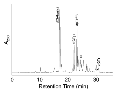
Figure 1. HPLC trace for the separation of the 254-nm irradiation mixture of d(GT_1^*) under anaerobic condition, in which d(GAbasic) , d(GTg) , and d(GT^{diH}) represent the dinucleoside monophosphate with the thymidine portion being replaced with an abasic site lesion, thymidine glycol, and 5-hydroxy-5,6-dihydrothymidine, respectively. “XL” designates the cross-link lesion.
