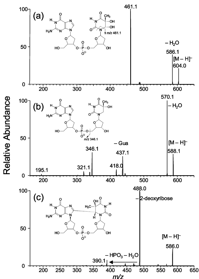
Figure 3. Product-ion spectra of the ESI-produced [M - H]^- ions of d(GT) (a), d(GT dih ) (b), and the XL (c).
