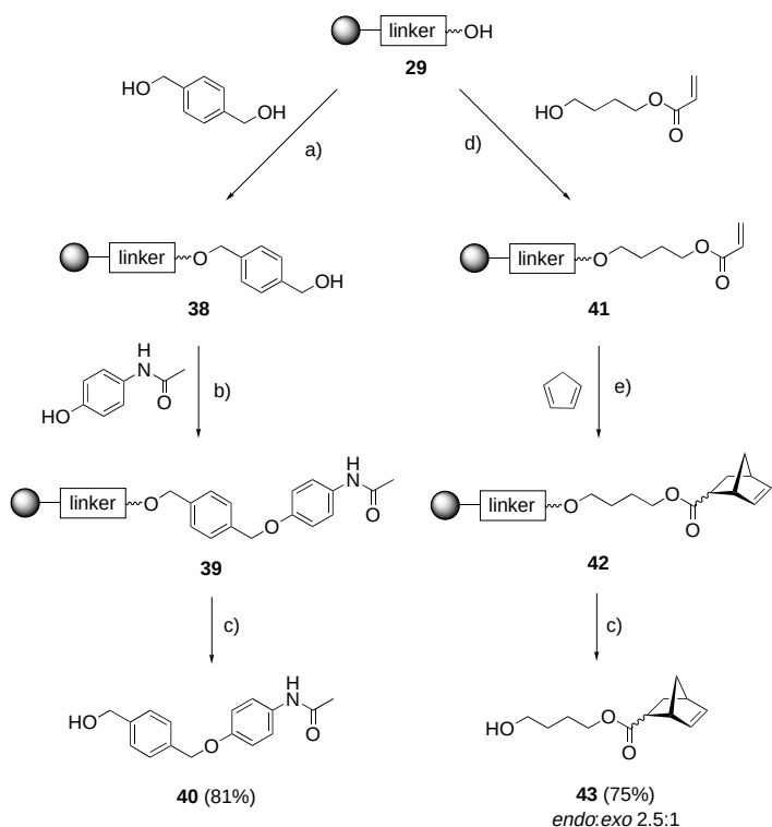
Scheme 8. Mitsunobu- and Diels–Alder reaction on polymeric support and penicillin G acylase mediated cleavage of the target molecules. a) DIC, DMAP, HOBT, DMF, pyridine, 0 °C, 1 h, then 20 °C, 24 h, 92 %; b) DEAD, PPh 3 , THF/CH 2 Cl 2 1:1, –5 °C, 2 h, then 20 °C, 20 h, 86 %; c) penicillin G acylase, pH 7.0, 10 % MeOH, 37 °C, 48 h; d) DIC, DMAP, HOBT, DMF, pyridine, 0 °C, 1 h, then 20 °C, 24 h, 97 %; e) THF, 60 °C, 15 h, 93 %.
