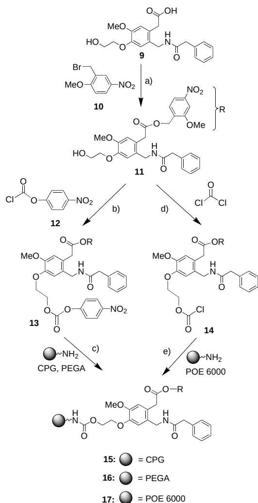
Scheme 3. Synthesis of polymer-bound linker 2-methoxy-5-nitrophenyl esters 15–17 . a) 10 , \text{Cs}_2\text{CO}_3 , \text{H}_2\text{O}/\text{EtOH} then DMF, rt, 82%; b) 12 , DMAP, \text{CH}_2\text{Cl}_2 , rt, 61%; c) CPG- \text{NH}_2 or PEGA- \text{NH}_2 , HOBT, EtN( i Pr) _2 , DMF, quant.; d) phosgene, \text{CH}_2\text{Cl}_2 , rt, quant.; e) POE- \text{NH}_2 , DMAP, HOBT, \text{CH}_2\text{Cl}_2 , rt, 92%. HOBT = 1-hydroxybenzotriazole, DMAP = 4-dimethylaminopyridine.
