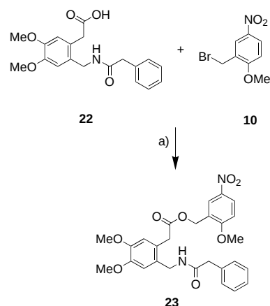
Scheme 5. Synthesis of model ester 23 . a) \text{Cs}_2\text{CO}_3 , DMF, rt, 68%.
