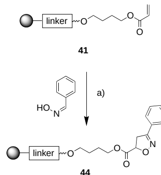
Scheme 9. 1,3-Dipolar cycloaddition to give the isoxazoline 44 . a) 0.7 M NaOCl, THF, 20 °C, 4 h, 94 %.
