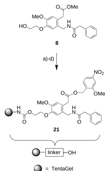
Scheme 4. Synthesis of TentaGel-bound 2-methoxy-5-nitrophenyl ester 21 . a) 12 , DMAP, \text{CH}_2\text{Cl}_2 , 0°C, 1 h then 20°C, 24 h, 48% ( \rightarrow 18 ); b) TentaGel- \text{NH}_2 , HOBT, DMF, 20°C, 10 h, quant. ( \rightarrow 19 ); c) 0.5 M LiOH/ \text{CH}_3\text{OH} 1:1, 20°C, 2 h, quant. ( \rightarrow 20 ); d) 10 , \text{Cs}_2\text{CO}_3 , DMF, rt, 81%.
