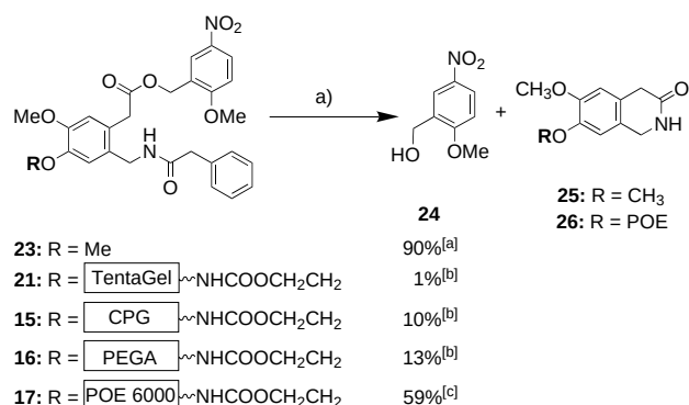
Scheme 6. Enzyme-initiated cleavage of 2-methoxy-5-nitro benzyl alcohol ( 24 ) from different polymeric supports and in solution; a) penicillin G acylase, conditions; [a] immobilized penicillin G acylase, 20% acetone, dimethyl- \beta -cyclodextrin, 37°C; [b] penicillin G acylase suspension, 10% methanol, 37°C; [c] penicillin G acylase suspension, 10% methanol, 20°C.
