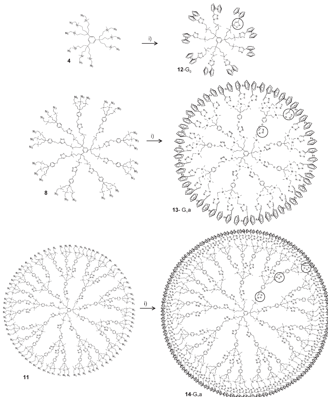
Scheme 2. Synthesis of the 1,2,3-triazolylferrocenyl dendrimers by “click Chemistry”. i) \text{CuSO}_4 , sodium ascorbate, \text{THF}/\text{H}_2\text{O} , RT, 30 min, ethynylferrocene.
