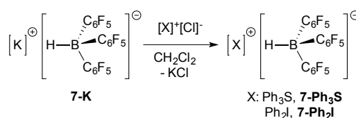
Scheme 4 Synthesis of hydrioborates 7-Ph 3 S and 7-Ph 2 I .
