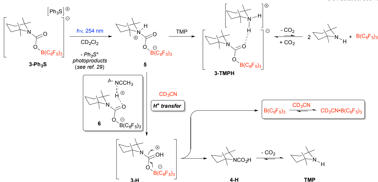
Scheme 3 Generation of 5 from 3-Ph 3 S under 254 nm light and suggested mechanism for photorelease of \text{B}(\text{C}_6\text{F}_5)_3 from 3-Ph 3 S in the presence of acetonitrile.
