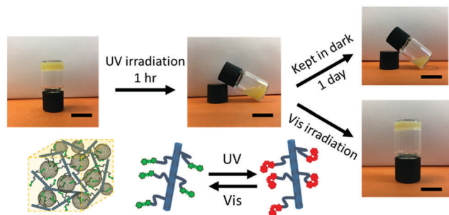
Fig. 4 Reversible photoswitching of a supramolecular hydrogel composed of 2.5 wt% Fmoc-RGDS, 0.25 wt% Fmoc-RGDS-AAP and 50 \mu M of CDV (scale bar: 1 cm).
