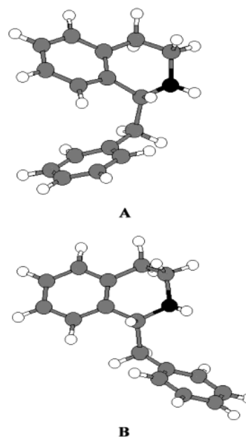
Figure 2. Semifolded (A) and extended (B) conformers of benzyltetrahydroisoquinoline, conformations optimized at the ab initio RHF-631g [d,p] level.
