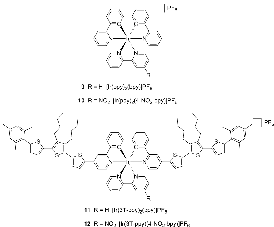
Figure 1. Molecular structures of cationic Ir(III) bis-cyclometalates. Control complexes 9 , 10 , and 3T-pendant complexes 11 , 12 .
