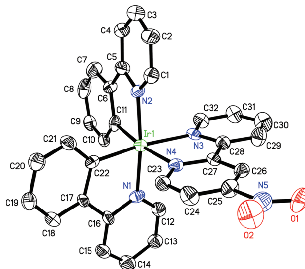
Figure 2. Thermal ellipsoid plot of [Ir(ppy) 2 (4-NO 2 -bpy)]PF 6 ( 10 ). Major component of disordered NO 2 substituent is shown. Hydrogen atoms and PF 6 − counterion have been removed for clarity.
