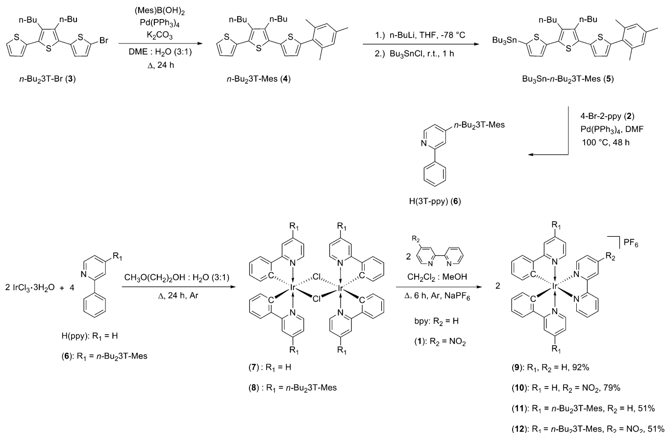
Scheme 1. Synthesis of 3T-Ligand and Cationic Ir(III) Bis-Cyclometalates
