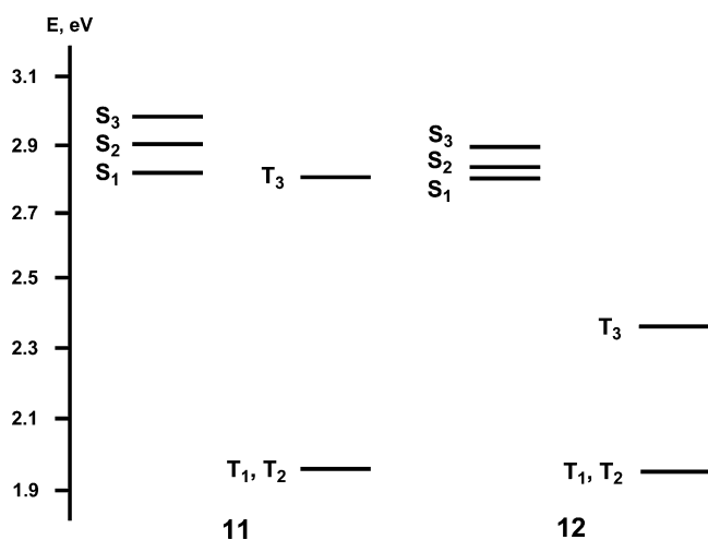
Figure 6. Energy level diagram for the lowest excited states in the 3T-pendant complexes ( 11–12 ).
