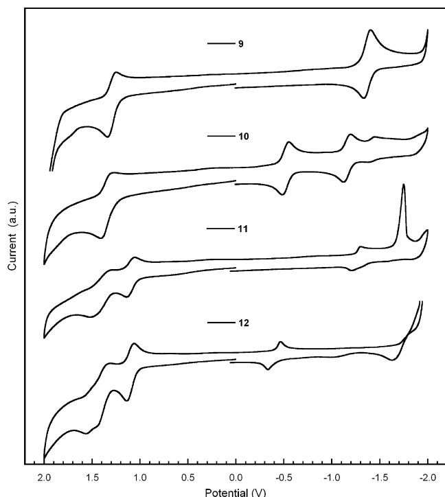
Figure 4. Cyclic voltammograms in ACN for control complexes 9 , 10 and 3T-pendant complexes 11 , 12 . Anodic currents are positive and plotted downward. Scan rate of 100 mV/s.
