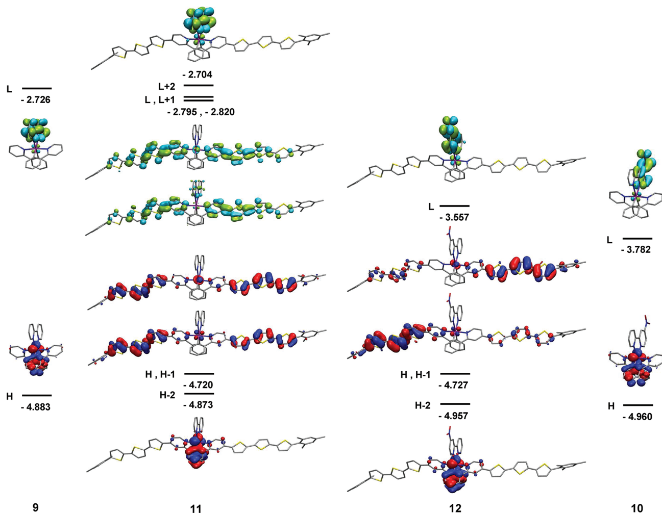
Figure 3. Contour plots of frontier orbitals (0.002 au) for control complexes ( 9–10 ) and 3T-pendant complexes ( 11–12 ) in the ground state. Occupied orbitals are shown in blue/red, virtual orbitals are in cyan/green. Hydrogen atoms omitted for clarity.
