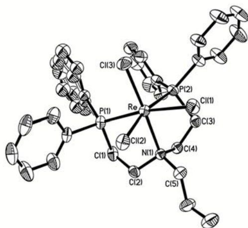
Fig. 6 ORTEP view of complex 4 . Thermal ellipsoids were drawn at the 40% probability level, with hydrogen atoms omitted for clarity. Bonds with alternate positions of atoms in the disordered phenyl ring were drawn in white, with disordered atoms refined only isotropically.
