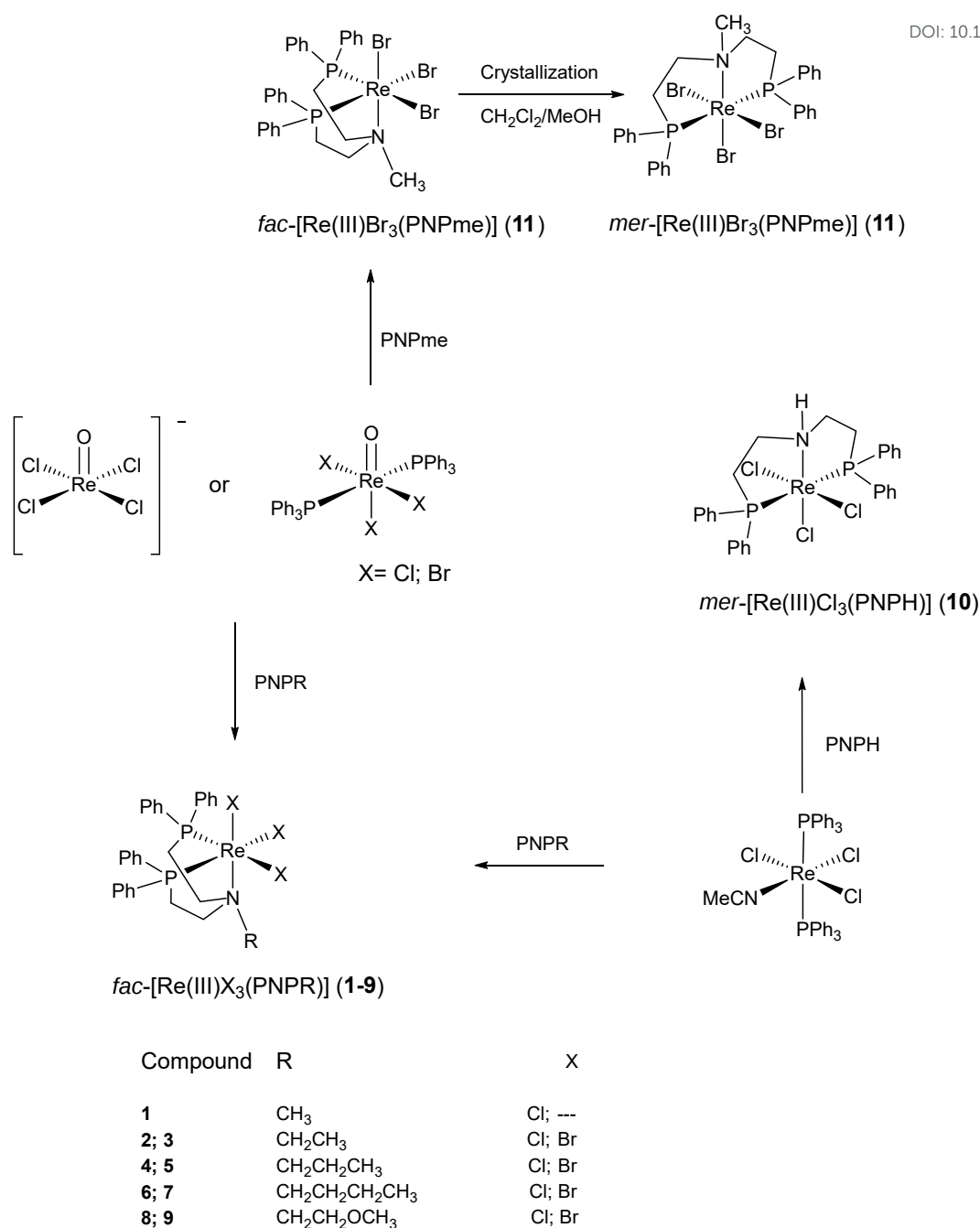
Scheme 1 Reactivity of the PNP ligands towards different rhenium(V) and rhenium(III) precursors.
