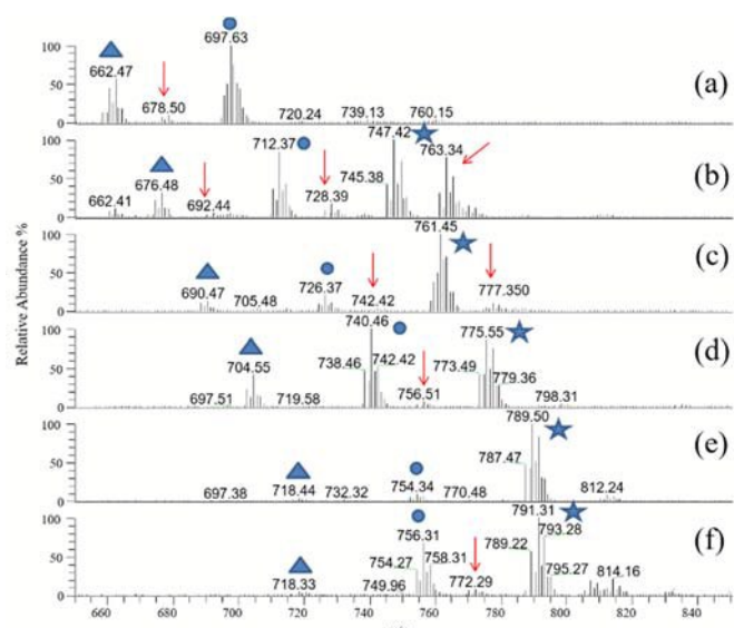
Fig. 3 Partial full scan ESI(+)-MS spectra (range: 640 – 850 m/z ) of compounds 10 (a), 1 (b), 2 (c), 4 (d), 6 (e) and 8 (f). Red arrows indicates the putative oxo-rhenium(V) ions as discussed in the main text. [★] = [\text{ReCl}_3(\text{PNPR})+\text{H}]^+ ; [●] = [\text{ReCl}_3(\text{PNPR})+\text{H}-\text{HCl}]^+ ; [▲] = [\text{ReCl}_3(\text{PNPR})+\text{H}-2\text{HCl}]^+ .
