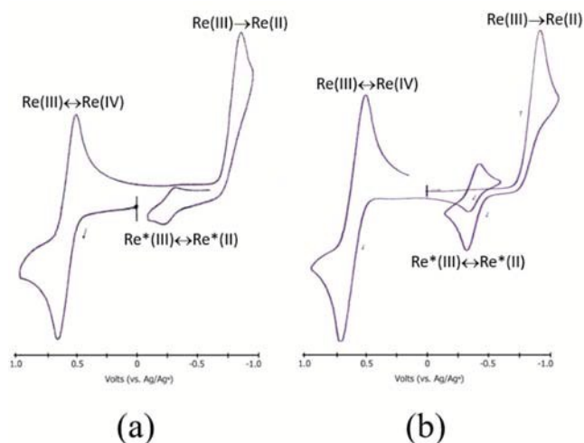
Fig. 1 Cyclic voltammograms of complexes 7 (a) and 8 (b). Data recorded at 200 mV s -1 , in dry and degassed dichloromethane with [n-Bu 4 N][ClO 4 ] (0.1 M) as supporting electrolyte, a platinum-disk working electrode, and a silver-wire quasi-reference electrode. Here, peaks are referred to the Ag/Ag + couple. Voltammetric data internally referred to the Fc/Fc + couple are given in Table 2.
