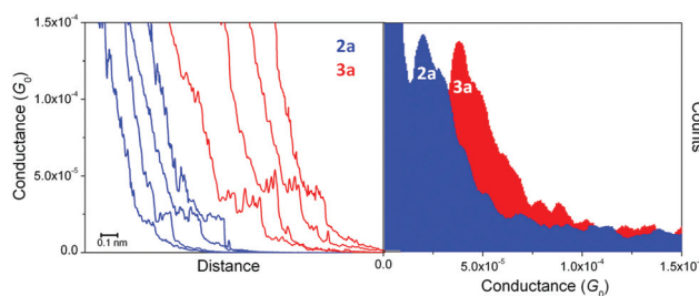
Fig. 3 Typical conductance traces from 2a and 3a using the I(s) method and conductance histograms derived from I(s) measurements. The curves are shifted horizontally for clarity. Conductance data are presented in units of the conductance quantum G_0 = 2e^2/h = 77.5 \mu\text{S} . I_0 = 20 nA and U_t = 0.6 V.
