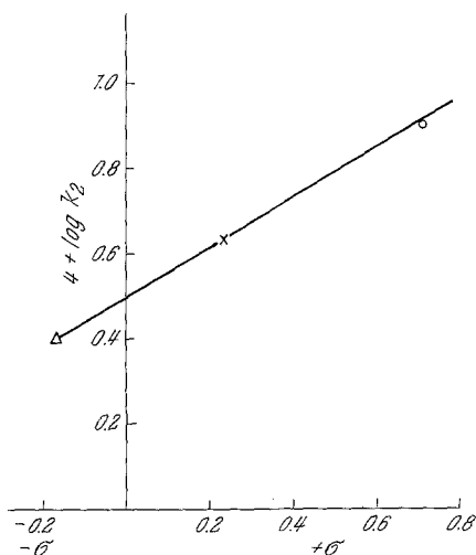
Fig. 3. Plot of \log k_2 versus Hammett substituent constants at 40^\circ . \bigcirc m = nitroacetophenone; \times p -chloroacetophenone; \Delta p -methylacetophenone
