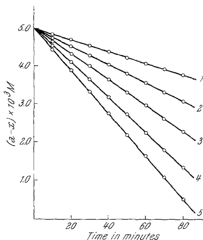
Fig. 1. Zero order rate plots at 40°. [ NBS ] = 1.0 \times 10^{-3}M , [ \text{HClO}_4 ] = 0.16M , [ \text{Hg}(\text{OAc})_2 ] = 2.0 \times 10^{-3}M , [ p -Me-PhCOMe] = 0.6, 1.0, 1.4, 1.8 and 2.2 \times 10^{-2}M in 1, 2, 3, 4 and 5 respectively
