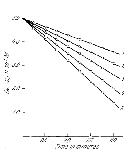
Fig. 2. Zero order rate plots at 40^\circ . [NBS] = 1.0 \times 10^{-3} M ; [p\text{-Me-PhCOMe}] = 1.0 \times 10^{-2} M ; [Hg(OAc)_2] = 2.0 \times 10^{-3} M ; [HClO_4] = 1.2, 1.6, 2.0, 2.4 and 2.8 \times 10^{-1} M in 1, 2, 3, 4 and 5 respectively
