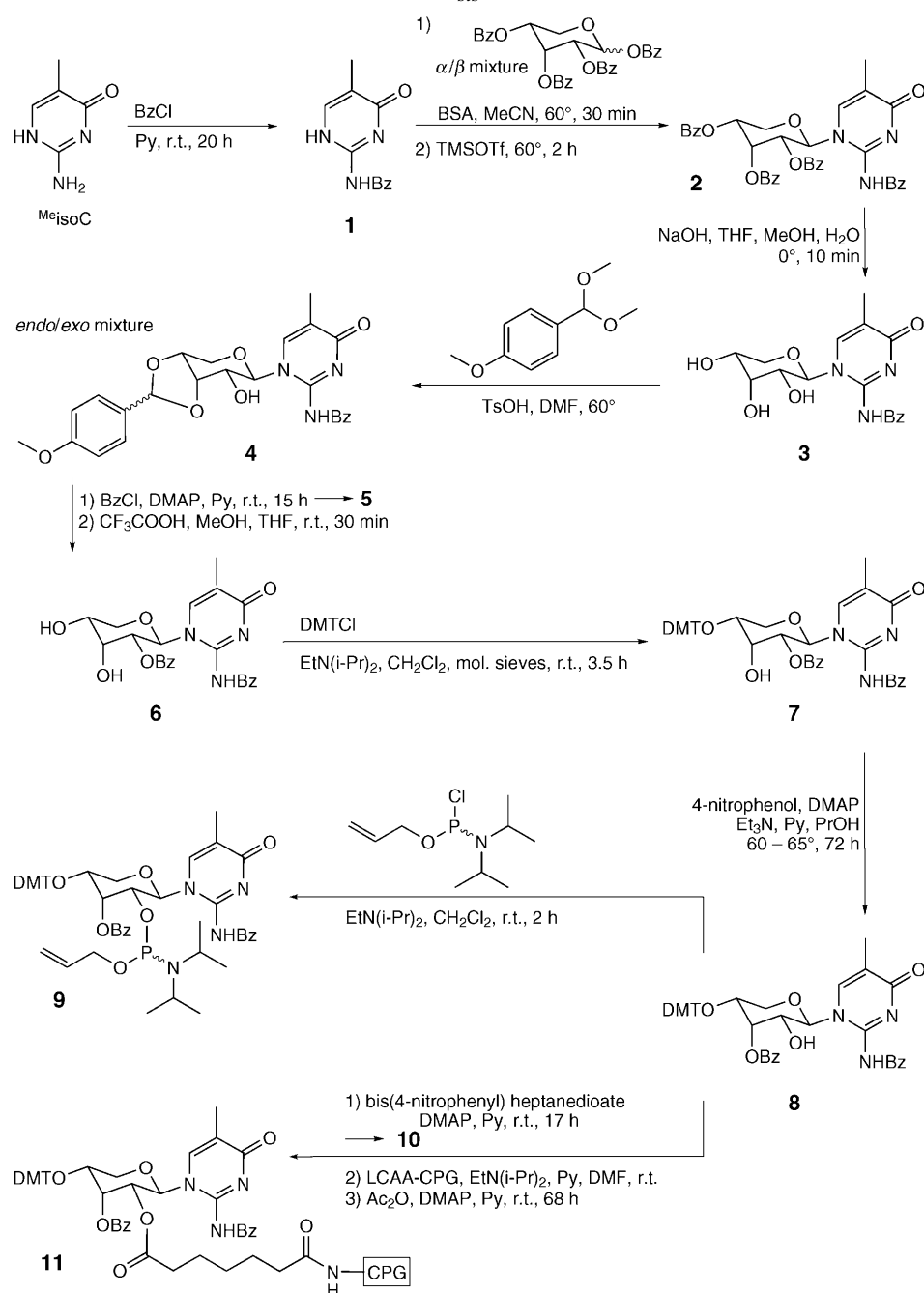
Scheme. Preparation of isoC Building Block 9 and Solid-Phase-Bound Unit 11 for Automated Synthesis
