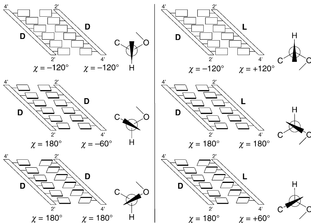
Fig. 4. Changes of nucleosidic torsion angle \chi and their consequences for pairing of isochiral (left) and heterochiral (right) strands. View for Newman projections is from the duplex centre outwards, in plane with bases (black wedge).
