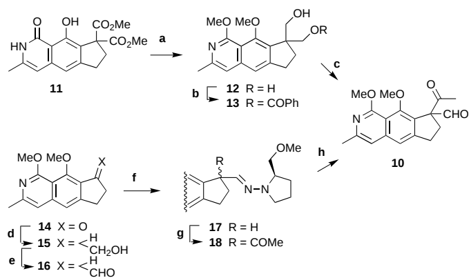
Scheme 4. Synthesis of the key intermediate 10 . a) 1. MeI, Ag 2 O, dioxane, 2. LiAlH 4 , THF, 35% for two steps; b) BzCl, pyridine, CH 2 Cl 2 , 45%; c) 1. Dess–Martin periodinane, MeCN, 2. MeMgBr, THF, then MeLi, 93% for two steps, 3. DMSO, (COCl) 2 , Et 3 N, CH 2 Cl 2 , 80%; d) 1. (Me) 3 Ph 3 P + Br − , t BuOK, THF, 83%. 2. BH 3 ·THF, THF then H 2 O 2 , 2N NaOH, 92%; e) Dess–Martin periodinane, CH 2 Cl 2 ; f) ( R )-1-amino-2-(methoxymethyl)-pyrrolidine, CH 2 Cl 2 , 87% for two steps; g) LDA, AcCl, THF, 77%; h) aqueous (CO 2 H) 2 , Et 2 O, 99%.
