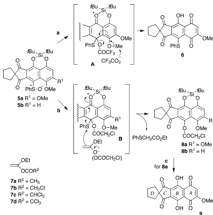
Scheme 3. Aromatic Pummerer-type reaction of 5 . a) (CF 3 CO) 2 O, styrene, CHCl 3 , 0 °C, 71 %; b) 7b , cat. p -TsOH, toluene, 110 °C, 72 % for 8b ; c) 1. Bu 4 NF, THF/H 2 O, room temperature, 2. BBr 3 , CH 2 Cl 2 , –78 → –45 °C, 3. 80 % CF 3 CO 2 H, reflux, 62 % from 5a .
