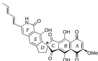
Figure 1. Fredericamycin A ( 1 ).
