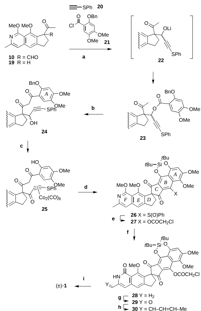
Scheme 5. Synthesis of racemic fredericamycin A ( 1 ). a) 20 , 21 , LiN(TMS) 2 , THF, 69%; b) LiN(TMS) 2 , toluene then HMPA, 70%; c) 1. Dess–Martin periodinane, CH 2 Cl 2 , 2. Co 2 (CO) 8 , CH 2 Cl 2 , 84% for two steps, 3. BCl 3 , CH 2 Cl 2 , 37%; d) 1. Me 2 SiCl 2 , Et 3 N, chloranil, toluene, 2. t Bu 2 Si(OTf) 2 , Et 3 N, DMF, 3. m CPBA, CH 2 Cl 2 , 47% for three steps; e) 7b , cat. p -TsOH, toluene, 77%; f) t Bu 2 Si(OTf) 2 , Et 3 N, MeI, DMF, quant.; g) SeO 2 , dioxane, 78%; h) (MeCH=CHCH 2 )Ph 3 P + Br − , n BuLi, THF, 28% (85% based on consumed 29 ); i) 1. BBr 3 , CH 2 Cl 2 , 2. THF/H 2 O, air, 3. HPLC separation, 52% for three steps.
