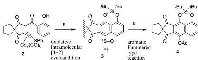
Scheme 2. Synthesis of the ABCD-ring precursor compound 4 . a) 1. Me 2 -SiCl 2 , Et 3 N, chloranil, 100 °C, 2. t Bu 3 Si(OTf) 2 , Et 3 N, 3. m CPBA; b) 1. (CF 3 CO) 2 O, styrene, 2. Ac 2 O, AcONa, pyridine.
