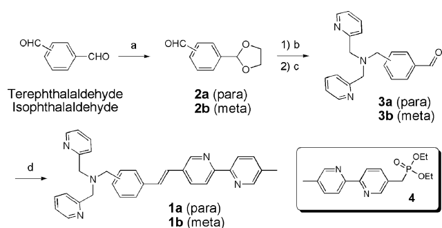
Scheme 1 Synthesis of 1a and 1b . Reagents and conditions: a. ethylene glycol, TsOH (cat.), Dean–Stark, reflux, 4 h; b. di(2-picoly)amine, NaBH(OAc) 3 , rt, 6 h; c. HCl–THF–H 2 O, rt, 14 h; d. NaH, dimethoxyethane, 4 , rt, 14 h.
