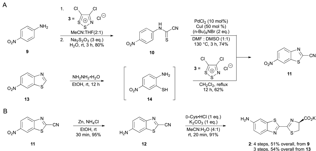
Scheme 5 Synthesis of aminoluciferin 2 . (A) Cyanobenzothiazole intermediate 11 was accessed via palladium-mediated cyclization (top) or metal-free cyclization (bottom). (B) A reduction-condensation sequence was used to prepare 2 .
