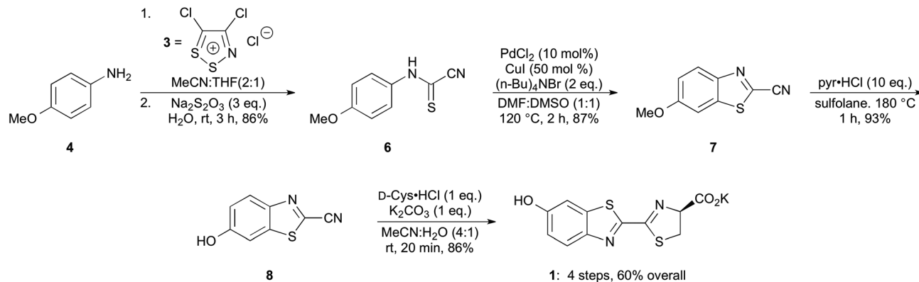
Scheme 3 Synthesis of D-luciferin (1) using an initial one-pot condensation/fragmentation procedure.
