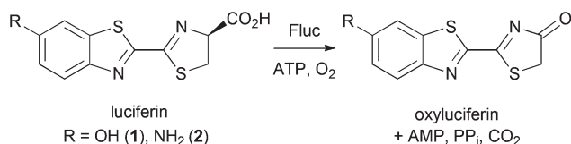
Fig. 1 Firefly luciferase (Fluc) catalyzes the oxidation of D-luciferin (1), its native substrate, and various analogs, including the 6'-amino compound (2). Light is produced during the enzymatic reactions.
