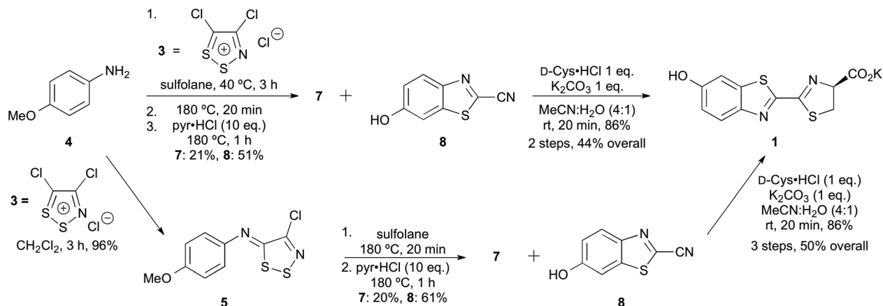
Scheme 4 Synthesis of D-luciferin (1) via Appel's salt condensation and thermolysis. The iminodithiazole adduct 5 can be isolated following treatment of p -anisidine (4) with Appel's salt (lower) or carried on directly into the cyclization and deprotection steps (upper).
