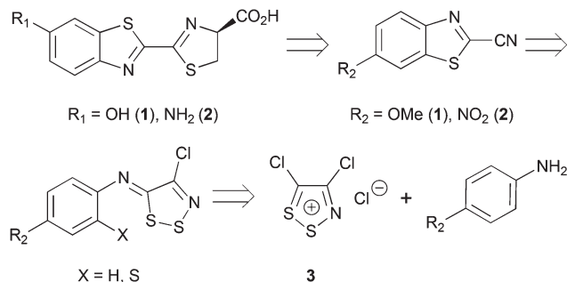
Scheme 1 Retrosynthetic analysis of D-luciferin (1) and its 6' amino analogue (2). Both molecules can be accessed from aniline starting materials and Appel's salt (3).
