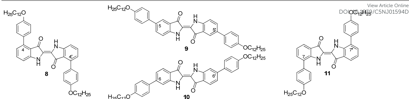
Figure 3. The four symmetrically 4-dodecyloxyphenyl-bissubstituted indigo-derivatives 8-11.
