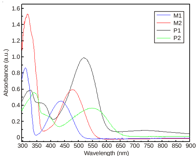
Fig. 2. UV-visible absorption spectra of M1, M2, P1 and P2 in \text{CHCl}_3 solution
