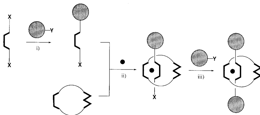
Figure 4. Principle of the synthesis of rotaxane 10a (see Figure 5): i) formation of a monostoppered axle; ii) threading of the axle through the wheel; iii) dethreading of the macrocycle is prevented by adding a second blocking group.
