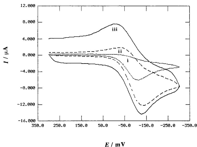
Figure 8. Illustration of the evolution of the CV curves of 10_{(5)}^{2+} when increasing the potential sweep rate (same conditions as indicated in Figure 7). i) v = 500 \text{ mVs}^{-1} , ii) v = 3000 \text{ mVs}^{-1} , iii) v = 8000 \text{ mVs}^{-1} .
