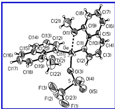
Figure 1. ORTEP drawing of 6 .
