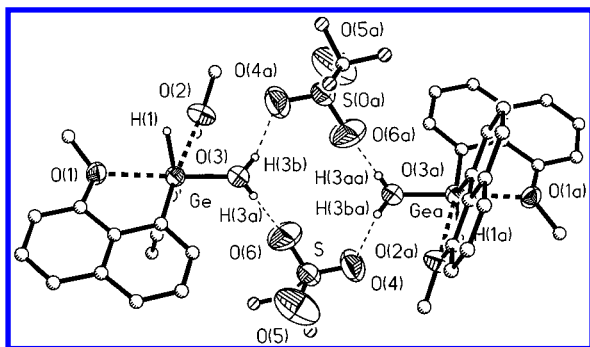
Figure 2. ORTEP drawing of 11 .
