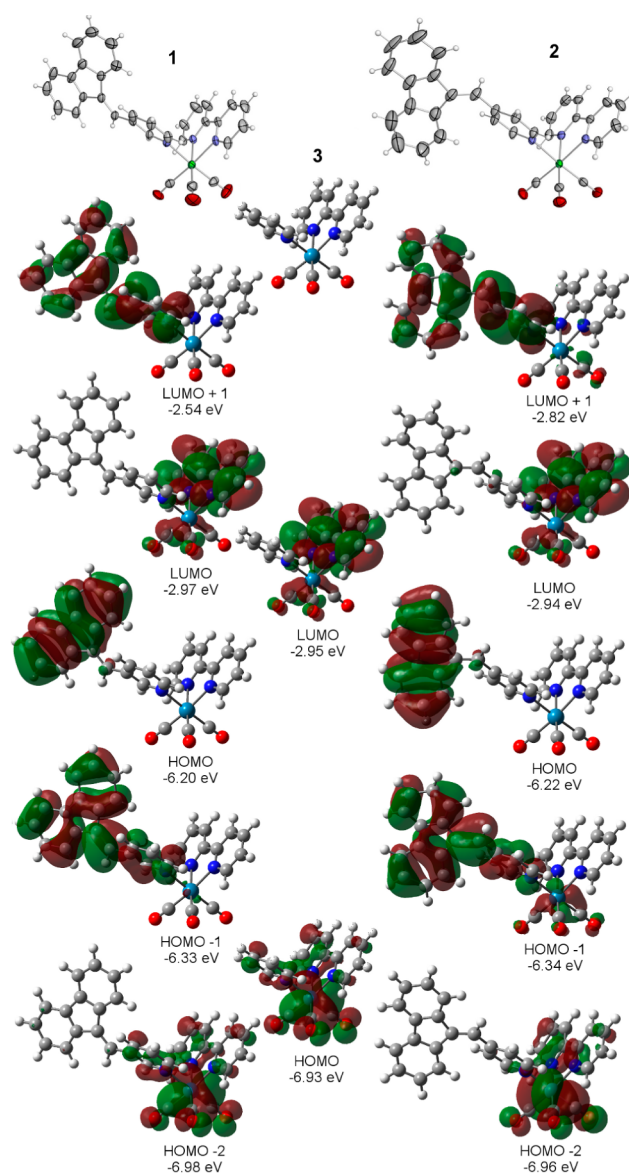
Figure 4. Topmost: ORTEP X-ray crystal structure of 1 (left) and 2 (right) used as starting point for the geometry optimization (50% probability displacement ellipsoids, anion, solvent and other chemically equivalent molecule removed); Top center: optimized structure of 3 starting from crystallographic data. 31 Middle: Frontier molecular orbitals and orbital energies obtained from DFT (rb3lyp/LanL2DZ(f)[Re]6-31G**[C,H,N,O]) CPCM(CH 2 Cl 2 ).
