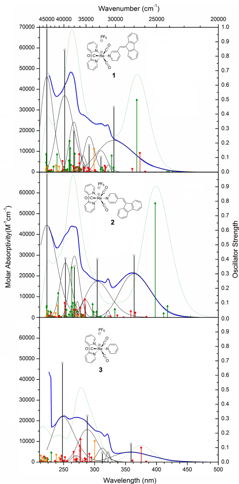
Figure 2. Absorption spectra in dichloromethane of the complexes (in blue; Top: 1 ; middle: 2 ; bottom: 3 ); Gaussian fits and sum of fits (black; full and dashed); Calculated curves from TD-DFT (dotted green); fitted oscillator strength (black circle); calculated from TD-DFT oscillator strength: Rhenium centered (red disk), Fulvene/pyridine centered (green triangle), bipyridine centered (orange triangle).
