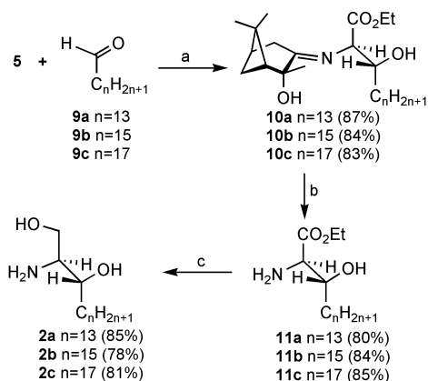
Scheme 2 Reagents and conditions: (a) \text{CITi}(\text{OEt})_3 , \text{NEt}_3 , \text{CH}_2\text{Cl}_2 , 0^\circ\text{C} ; (b) 1N \text{HCl} , THF; (c) \text{LiAlH}_4 , THF, reflux.
