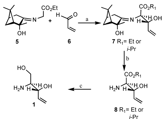
Scheme 1 Reagents and conditions: (a) \text{CITi}(\text{OEt})_3 , \text{NEt}_3 , \text{CH}_2\text{Cl}_2 , 0^\circ\text{C} , 72% or \text{CITi}(\text{OPr-}i)_3 , \text{NEt}_3 , \text{CH}_2\text{Cl}_2 , 0^\circ\text{C} , 70%; (b) 1N \text{HCl} , THF, 82%; (c) 2M \text{LiBH}_4 , THF–MeOH, 74%.
