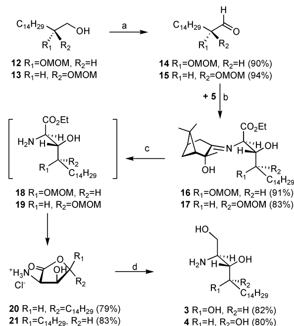
Scheme 3 Reagents and conditions: (a) Dess–Martin periodinane, \text{CH}_2\text{Cl}_2 , Py, RT; (b) \text{CITi}(\text{OEt})_3 , \text{NEt}_3 , \text{CH}_2\text{Cl}_2 , 0^\circ\text{C} ; (c) 1N \text{HCl} , THF, RT; (d) \text{LiAlH}_4 , THF, reflux.
