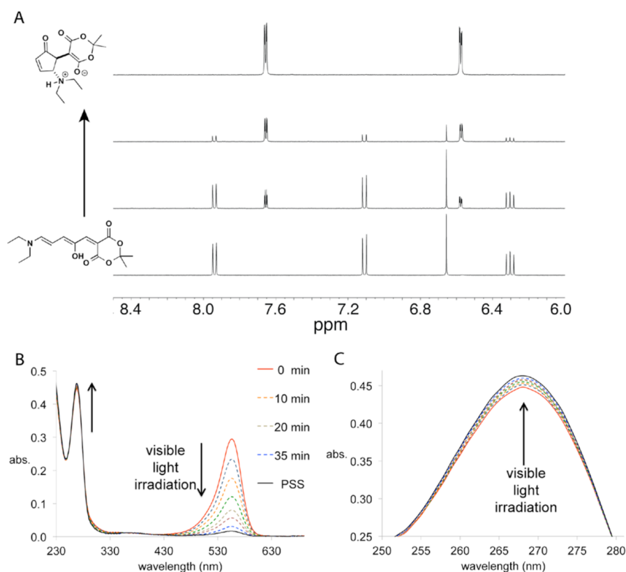
Figure 7. (A) The conversion of 22 to 73 by 1 H NMR in CD 3 OD over 4 h. (B) Absorption spectra of 34 to 78 on irradiation with visible light ( \lambda = 570 nm) in methanol. (C) Expanded view of absorption spectra between 250–280 nm.
