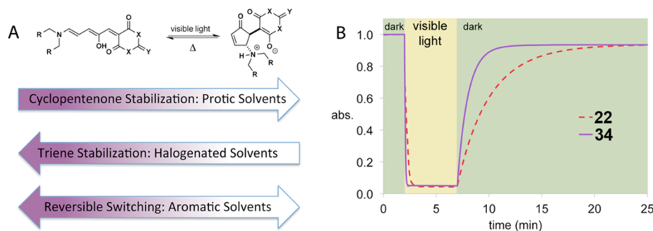
Figure 8. (A) Solution-state switching behavior of DASAs. (B) In situ kinetic plot of the switching cycle of 22 and 34 in PhMe, monitored at \lambda_{\text{max}} of 545 and 570 nm, respectively.
