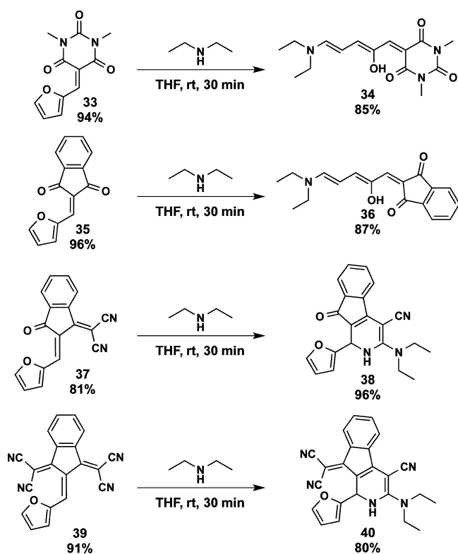
Scheme 2. Investigation of Furan Activating Groups for the Synthesis of DASAs
