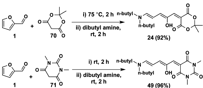
Scheme 3. One-Pot "On Water" Synthesis of DASAs
