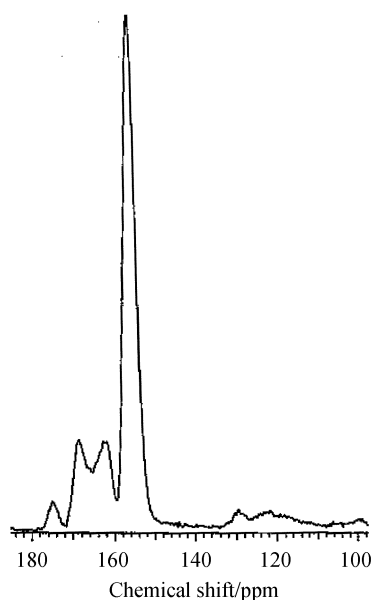
Fig. 1 A CP-MAS (6 K) carbon-13 NMR spectrum of the potassium phenoxide– 13 CO 2 complex in a sealed ampoule.
