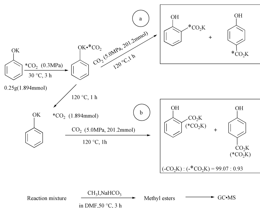
Scheme 3 Incorporation of carbon-13 in the reaction of potassium phenoxide-carbon dioxide complex
