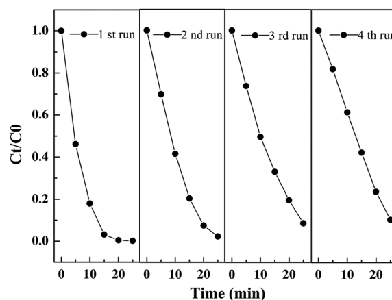
Fig. 9 Recycling test of BG5.0 in photocatalytic degradation of RhB.
