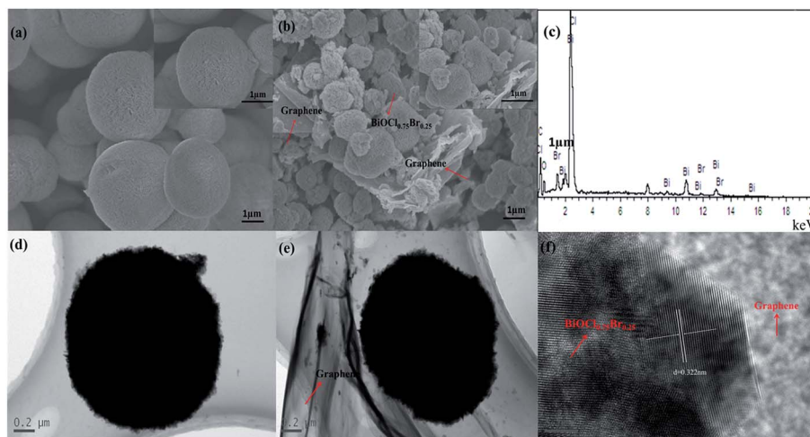
Fig. 2 FESEM and TEM image of (a), and (d) BiOCl 0.75 Br 0.25 , (b), and (e) BG5.0, (c) the EDX spectrum of BG5.0 and HRTEM (f) image of BG5.0.
