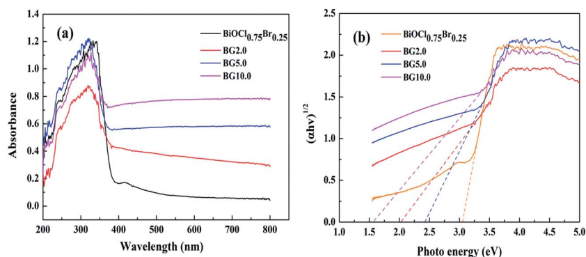
Fig. 4 (a) UV-vis diffuse reflectance spectra of the samples; (b) the band gaps ( E_g ) of different samples.
