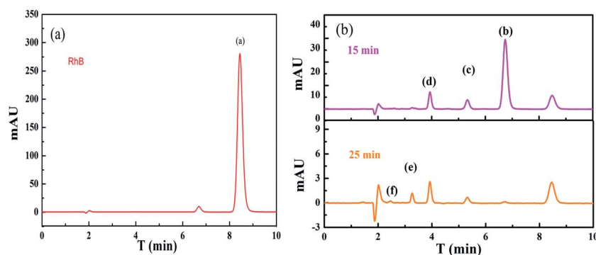
Fig. 7 HPLC chromatograms of the RhB (a) and (b) the N -deethylated intermediates recorded at 554 nm at 15 and 25 m.
