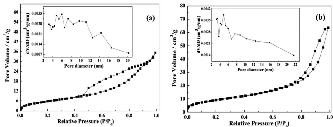
Fig. 5 \text{N}_2 adsorption and desorption isotherms of the (a) \text{BiOCl}_{0.75}\text{Br}_{0.25} (b) BG5.0. Insets: the corresponding pore-size distribution.
