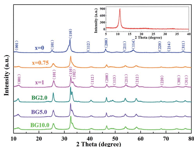
Fig. 1 XRD patterns of GO, \text{BiOBr} , \text{BiOCl}_{0.75}\text{Br}_{0.25} , \text{BiOCl} and \text{BiOCl}_{0.75}\text{Br}_{0.25} /graphene (BG2.0, BG5.0, BG10.0) samples.
