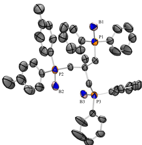
Fig. 2 ORTEP drawing of the borane-adduct 2-PG where all non-hydrogen atoms are represented by Gaussian ellipsoids at the 50 % probability level. All hydrogen atoms have been omitted for clarity.
