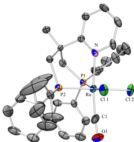
Fig. 4 ORTEP drawing of the dichloro ruthenium complex D-3 where all non-hydrogen atoms are represented by Gaussian ellipsoids at the 50 % probability level. All hydrogen atoms and coordinating solvent have been omitted for clarity. Selected bond lengths (Å) and angles (°) of D-3 : Ru–P1 = 2.2970(14); Ru–P2 = 2.2844(15); Ru–N = 2.178(4); Ru–Cl1 = 2.4314(13); Ru–Cl2 = 2.4775(14); P1–Ru–P2 = 87.65(5); P1–Ru–N = 83.76(11); P2–Ru–N = 90.25(11).
