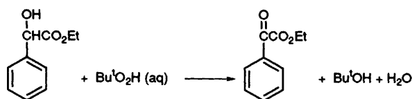
Scheme 1 Reagents and conditions: CuCl 2 (1 mol%), TBAB (3 mol%) CH 2 Cl 2 , 25 °C, 24 h, conversion 96%
