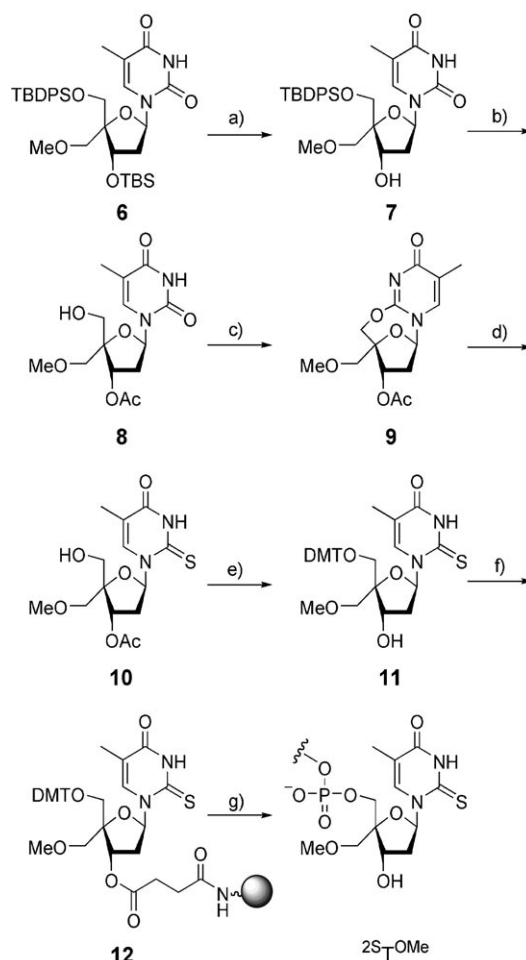
Scheme 2. a) \text{BF}_3 \cdot \text{Et}_2\text{O} , \text{CH}_2\text{Cl}_2 , 89%; b) 1. acetic anhydride, DMAP, pyridine; 2. TBAF, THF, 92%; c) 1. 2,6-lutidine, \text{TiF}_2\text{O} , DMF; 2. DBU, \text{CH}_3\text{CN} , 0^\circ\text{C} –RT; 75% over both steps; d) \text{H}_2\text{S} , pyridine, 45^\circ\text{C} , 28%; e) 1. DMTCI, DMAP, pyridine; 2. aq. \text{NH}_3 , MeOH; 40% over both steps; f) EDC, DMAP, succinylated LCAA-CPG, pyridine; then 4-nitrophenol; then piperidine; then acetic anhydride/pyridine/THF (Cap A) and 1-methylimidazole/THF (Cap B); g) 1. oligonucleotide synthesis; 2. 25% \text{NH}_4\text{OH} . DBU: 1,8-diazabicyclo[5.4.0]undec-7-ene; DMF: N,N -dimethylformamide; TBAF: tetrabutylammonium fluoride; \text{TiF}_2\text{O} : trifluoroacetic anhydride.
