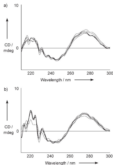
Figure 2. Circular dichroism spectra of native and modified oligonucleotides. Primer probes (20-mer) were hybridised with template (33-mer) in matched (A–T/T*) and mismatched (G–T/T*) cases. A) T match, T mismatch, ^{2S}T match, ^{2S}T mismatch, ^{4S}T match and ^{4S}T mismatch; B) T^{OMe} match, T^{OMe} mismatch, ^{2S}T^{OMe} match, ^{2S}T^{OMe} mismatch, ^{4S}T^{OMe} match and ^{4S}T^{OMe} mismatch. T*: modified thymidines ^{2S}T , ^{4S}T , T^{OMe} , ^{2S}T^{OMe} or ^{4S}T^{OMe} as described above.
