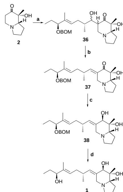
Scheme 7. Synthesis of (+)-allopumiliotoxin 323B' 1 . a) KHMDS, THF/HMPA, 0 °C then 7 ; b) DBU, TFAA, DMAP, –50 °C, CH 2 Cl 2 (42 %, two steps); c) Me 4 NBH(OAc) 3 , acetone, AcOH (89 %); d) LiDBB, THF, –78 °C (88 %).
