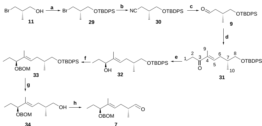
Scheme 5. Synthesis of the side chain, aldehyde 7 . a) TBDPSCI, DMF, imidazole (96 %); b) DMSO, NaCN, 120 °C (90 %); c) DIBAL, toluene, 0 °C (80 %); d) 8 , toluene, 90 °C (85 %); e) ( R )-CBS catalyst, \text{CH}_2\text{Cl}_2 , -40 °C, catecholborane (73 %); f) BOMCl, toluene, i\text{Pr}_2\text{EtN} , \text{Bu}_4\text{NI} , reflux (97 %); g) TBAF, THF (90 %); h) TPAP, NMO, \text{CH}_2\text{Cl}_2 (94 %).
