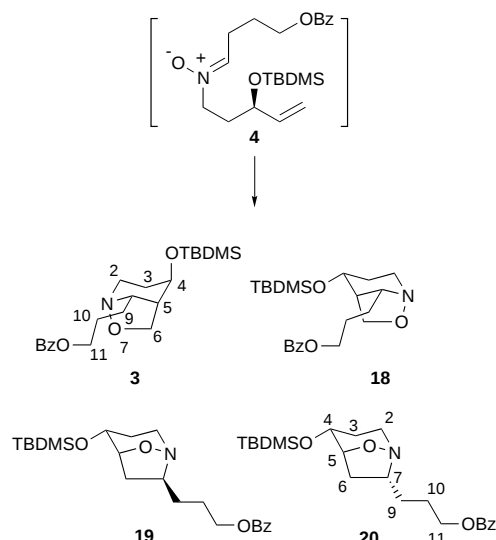
Scheme 3. Intramolecular [3 + 2]-cycloaddition reaction of ( Z )- N -alkenyl-nitron 4 . Toluene, 70^{\circ}\text{C} ( 3 , 32%; 18 , 5%; 19 , 8%; 20 , 8% from 16 ).
