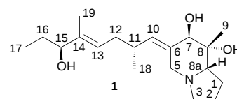
Figure 1. (+)-Allopumiliotoxin 323B' 1 .
