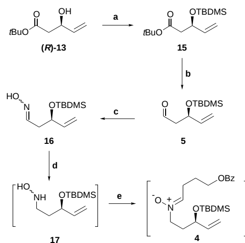
Scheme 2. Synthesis of ( Z )- N -alkenylnitrone 4 . a) TBDMSCl, imidazole, CH 2 Cl 2 (98 %); b) DIBAL, toluene, – 78 °C (79 %); c) H 2 NOH · HCl, H 2 O/EtOH, NaOAc (98 %); d) NaBH 3 CN, MeOH/HCl, MeOH; e) 6 , CH 2 Cl 2 .
