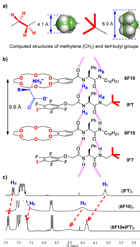
Figure 2. a) Computed molecular dimensionalities for methylene ( \text{CH}_2 ) and tert -butyl groups at the level of \omega\text{B97XD/6-311G}^{**} . b) Illustration of applying tert -butyl groups to alternatively interpenetrate the straight alkyl chains, generating more stable hetero-oligomeric peptidic ensembles as three-in-one transporters for transporting cations, anions and amino acids. c) Partial NMR spectra of homo-ensembles (\text{IFT})_n and (6\text{F10})_n and hetero-ensembles (6\text{F10-IFT})_n , demonstrating the formation of (6\text{F10-IFT})_n upon mixing (\text{IFT})_n and (6\text{F10})_n .
