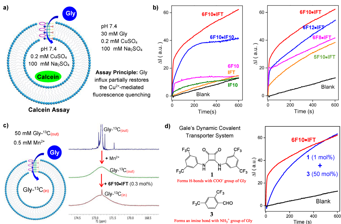
Figure 4. a) Illustration of amino acid-sensitive calcein assay for assessing the ability of amino acid transporters to transport glycine ( \lambda_{ex} = 495 nm, \lambda_{em} = 515 nm). b) Glycine transport curves for various channels at 20 μM. c) 13 C NMR spectra that verify the glycine transport by hetero-channel (6F10-IFT) 3 . d) Glycine transport curves for (6F10-IFT) 3 and Gale's dynamic covalent transporter system that employs 1 (1 mol %) and 3 (50 mol %).
