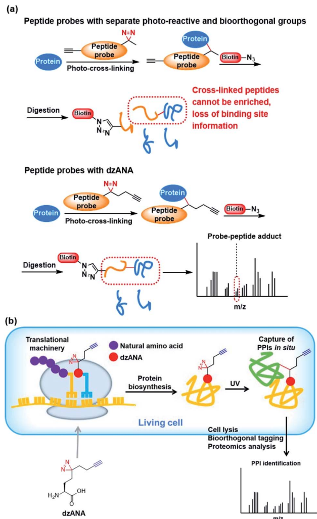
Fig. 5 Potential applications of dzANA in (a) mapping PPIs binding sites, and (b) study PPIs in living cells.
