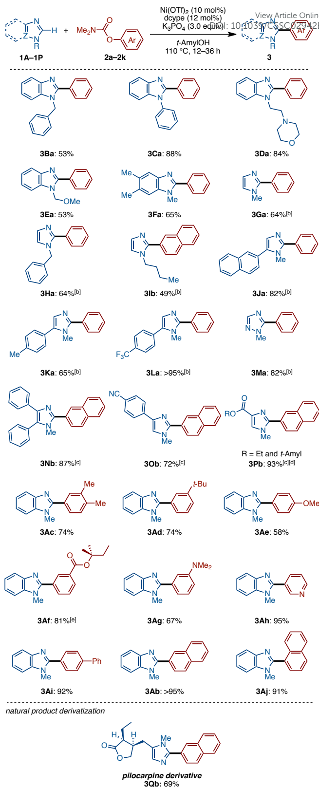
Scheme 1. Substrate scope of imidazole C–H arylation with phenol derivatives. [a] Unless otherwise noted, reaction conditions were as follows: 1 (0.40 mmol), 2 (1.5 equiv), \text{Ni}(\text{OTf})_2 (10 mol%), \text{dcype} (12 mol%), \text{K}_3\text{PO}_4 (3.0 equiv), t -AmylOH (1.6 mL), 110 °C, 12–36 h. [b] \text{Ni}(\text{cod})_2 (10 mol%) was used. [c] \text{Ni}(\text{cod})_2 (10 mol%) and \text{dcyp} (12 mol%) was used. [d] Starting from ethyl 4-imidazolecarboxylate 1P . (R = Et: 33%; t -Amyl: 60%). [e] Starting from methyl 3-((dimethylcarbamoyl)oxy)benzoate ( 2f ).
