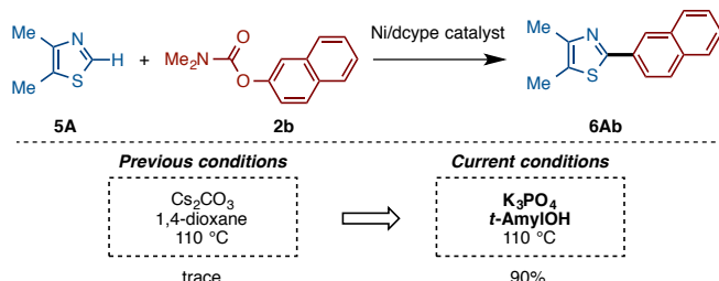
Scheme 5. Comparison of previous and current conditions for the reaction of thiazole 5A .
