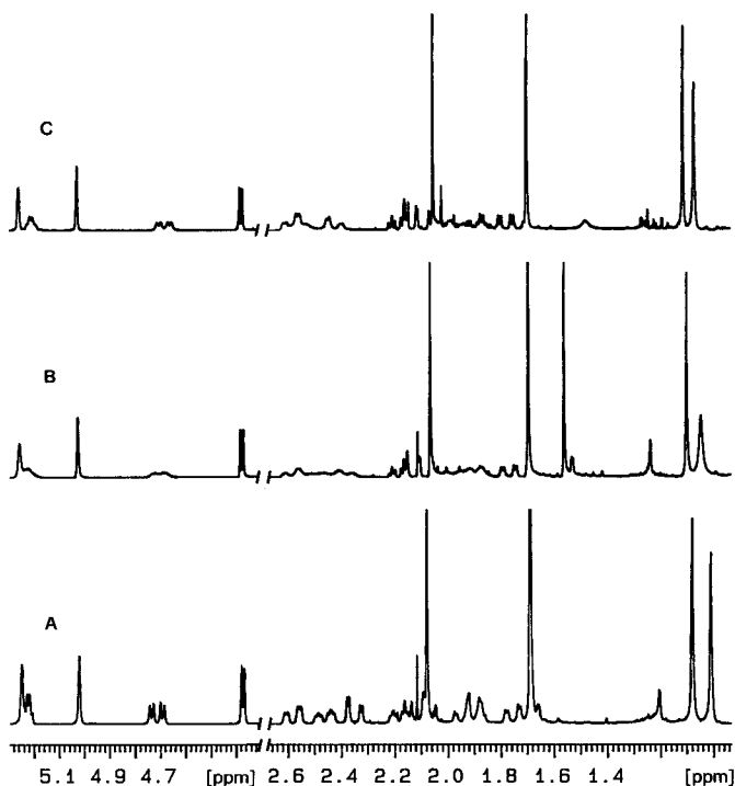
Figure. 300-MHz 1 H-NMR Spectra (CDCl 3 ) of rogiolol acetate ((+)- 3a ) at -30° (A), +21° (B), and +50° (C)
