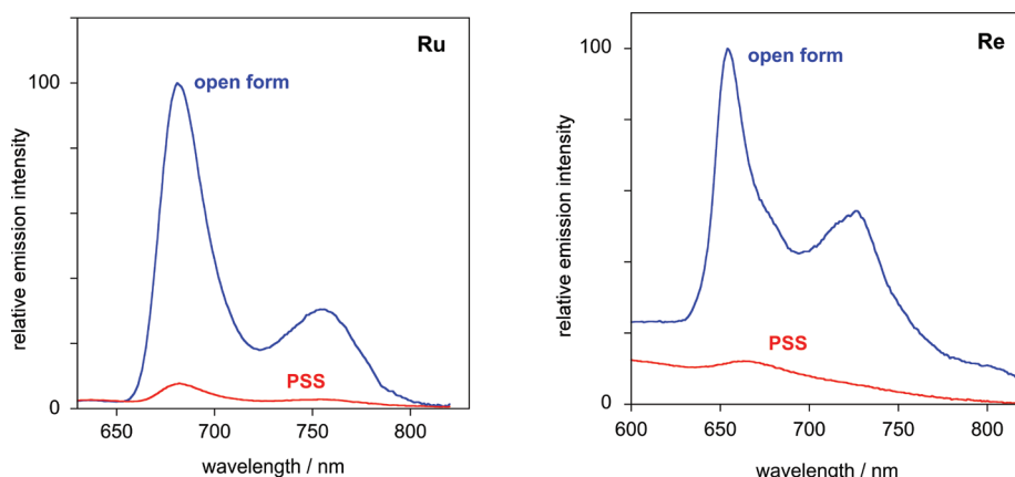
Figure 3. (left) Emission spectrum of [(L^a(o))(dmbipy)_2Ru](PF_6)_2 at 77 K in diethyl ether/isopentane/ethanol (2/2/1 v/v) (blue line) upon excitation into the lowest energy absorption band (490 nm) and the corresponding spectrum recorded for the photostationary state (red line). (right) Corresponding spectra of (L^a(o))Re(CO)_3Br and its PSS.
