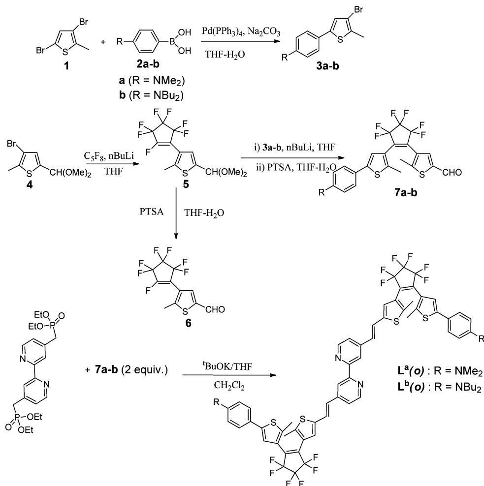
Scheme 2. Stepwise Synthesis of Photochromic Bipyridyl Ligands
