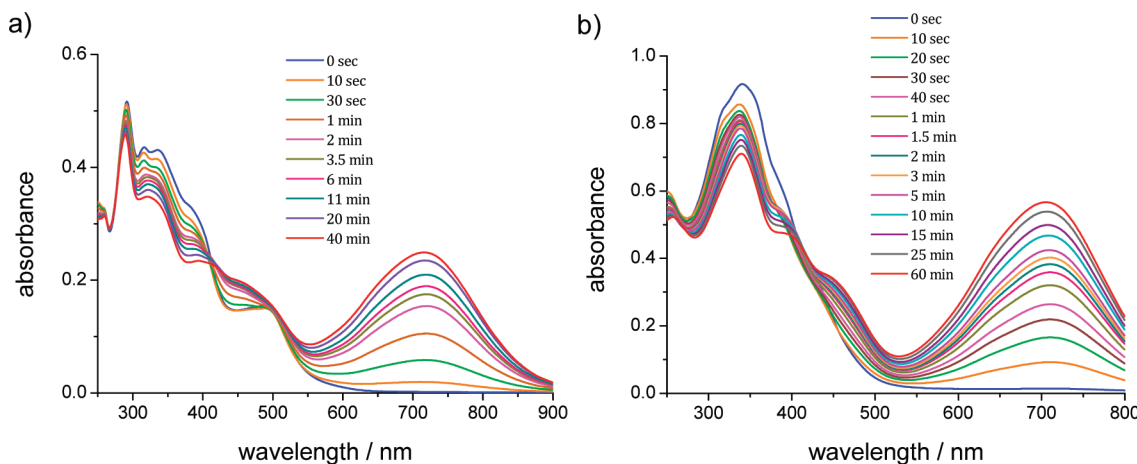
Figure 2. UV–vis absorption spectra changes of (a) [(\text{L}^{\text{a}})(\text{dmbipy})_2\text{Ru}](\text{PF}_6)_2 and (b) (\text{L}^{\text{a}})\text{Re}(\text{CO})_3\text{Br} in dichloromethane upon excitation at 350 nm.
