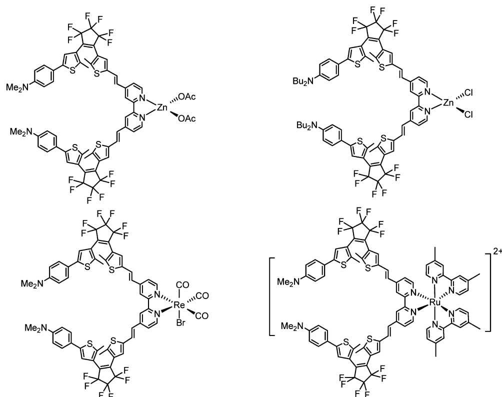
Figure 1. Chemical structures of photochromic bipyridine Zn(II), Re(I), and Ru(II) complexes.
