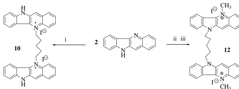
Scheme 2. Synthesis of bis-alkylated quindolines. Reagents: (i) trimethylene sulfone (TMS), \text{I}(\text{CH}_2)_5\text{I} ; (ii) NaH, \text{I}(\text{CH}_2)_5\text{I} ; (iii) \text{CH}_3\text{I} , TMS.
