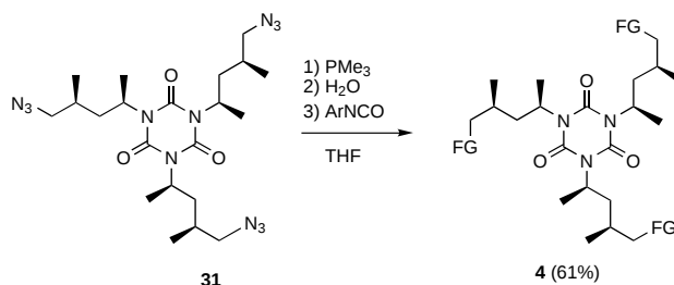
Scheme 11. Assembly of the side chains. Ar = n\text{C}_4\text{H}_9\text{-}p\text{C}_6\text{H}_4\text{-} ; FG = \text{NH-CO-NH-}p\text{C}_6\text{H}_4\text{-}n\text{C}_4\text{H}_9\text{-} .
