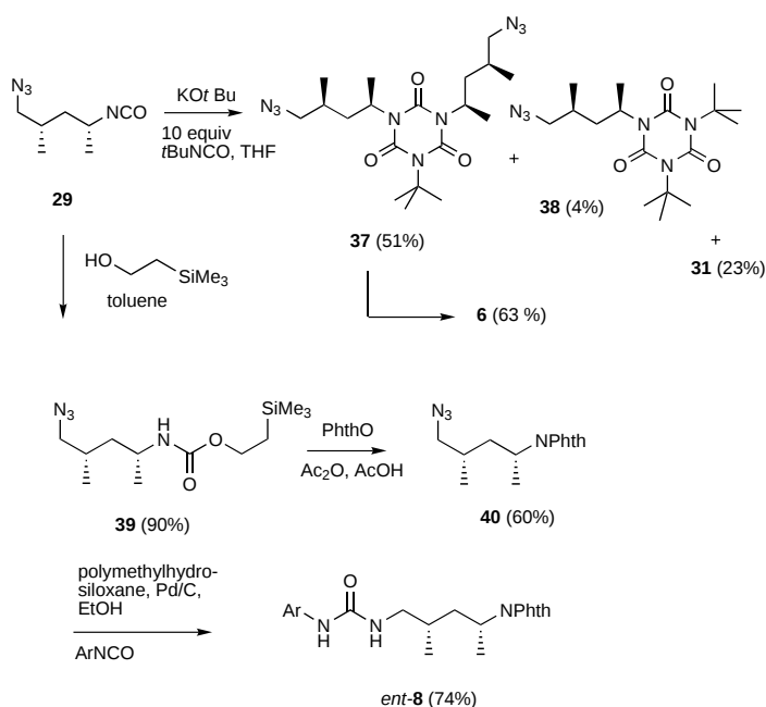
Scheme 12. Side chain modifications. Ar = n\text{C}_4\text{H}_9 - p\text{C}_6\text{H}_4 -.
