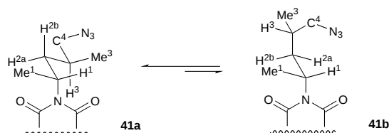
Scheme 13. Conformational equilibrium of 41 .
