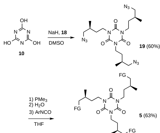
Scheme 6. Synthesis of host 5 . Ar = n\text{C}_4\text{H}_9\text{-}p\text{C}_6\text{H}_4\text{-} ; FG = \text{NH-CO-NH-}p\text{C}_6\text{H}_4\text{-}n\text{C}_4\text{H}_9 .
