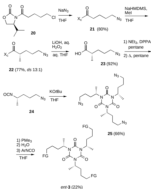
Scheme 7. Synthesis of host ent - 3 . Ar = n\text{C}_4\text{H}_9\text{-}p\text{C}_6\text{H}_4\text{-} ; FG = \text{NH-CO-NH-}p\text{C}_6\text{H}_4\text{-}n\text{C}_4\text{H}_9 .
