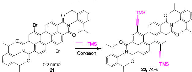
Scheme 4. Synthesis of PDI.
