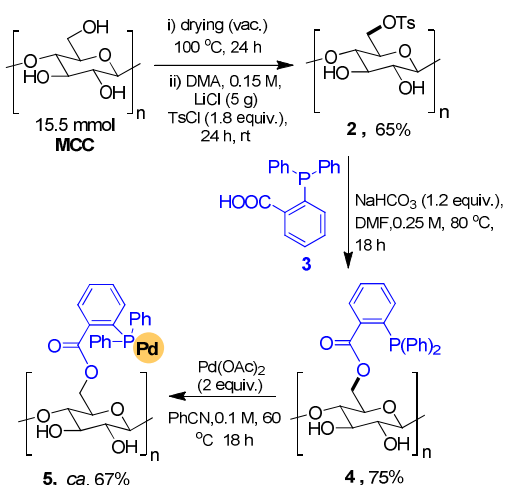
Scheme 2. Synthetic protocol of Cellulose-Pd NPs.
