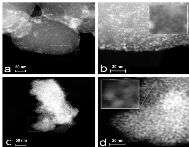
Figure 1. (a). Low-magnification STEM data from fresh catalyst; (b) Higher-magnification STEM images of regions marked in panel (a); (c). Low-magnification STEM data from five-times recycled catalyst; (d) Higher-magnification STEM images of regions marked in panels (c).
