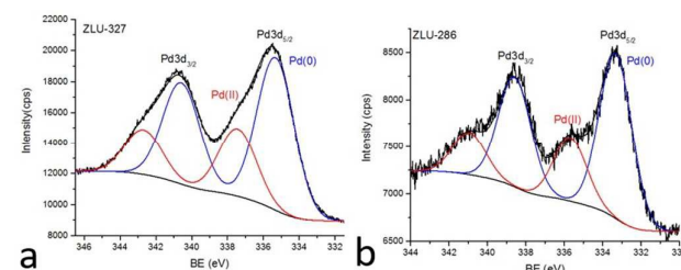
Figure 2. Deconvoluted high-resolution Pd3d XPS spectra. (a) XPS data of fresh catalyst; (b) XPS data of five-times recycled catalyst.
