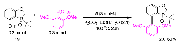
Scheme 3. Synthetic value of protocol.
