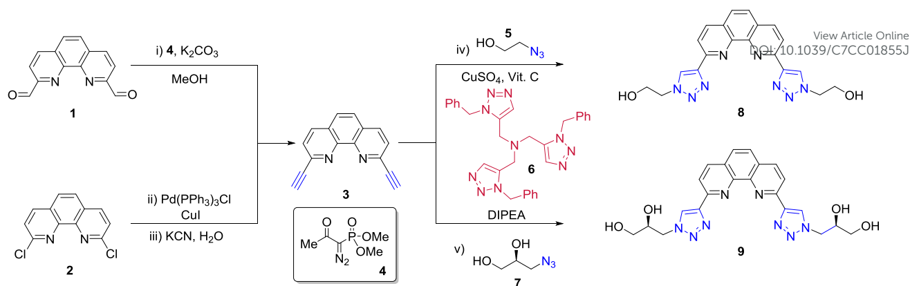
Scheme 1 Synthesis of hydrophilic, 2,9-bis-(1,2,3)-triazolyl-1,10-phenanthroline (BTrzPhen) ligands 8 and 9 .
