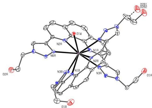
Fig. 2. Single crystal X-ray diffraction structure of the [\text{Eu}(\text{8})_2\text{OTf}_3] complex.
