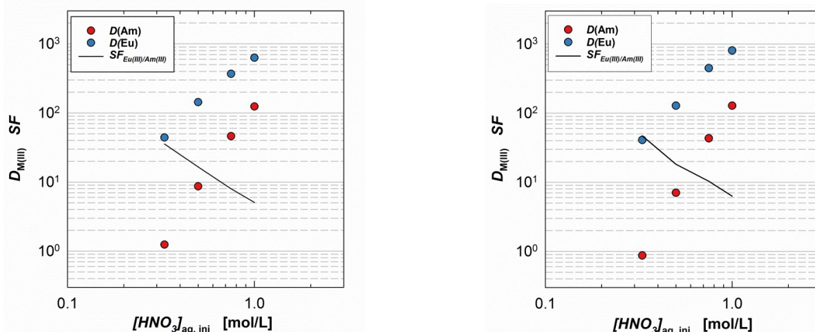
Fig. 1 Distribution ratios ( D_{M(III)} ) and separation factors ( SF_{Eu/Am} ) obtained in the extraction of ^{241}\text{Am(III)} and ^{152}\text{Eu(III)} by 8 (left) and 9 (right). Organic phase: TODGA (0.2 mol L^{-1} ) and 5 vol% 1-octanol in kerosene. Aqueous phase: HNO_3 (0.33–1.0 mol L^{-1} ) † and BTrzPhen ligands 8 and 9 (10 mmol L^{-1} ). Vortex Shaker (40Hz) for 12 hours at 20 \pm 0.5 \text{ } ^\circ\text{C} .
