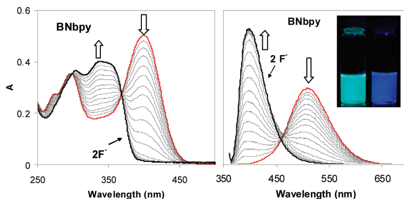
Figure 9. UV–vis (left) and fluorescent (right) spectral change of BNbpy ( \sim 1.0 \times 10^{-5} M) with the addition of NBu 4 F ( \lambda_{\text{ex}} = 350 nm). Inset: Photographs of the BNbpy solution before (left) and after (right) F − under UV irradiation (lamp wavelength 365 nm).
