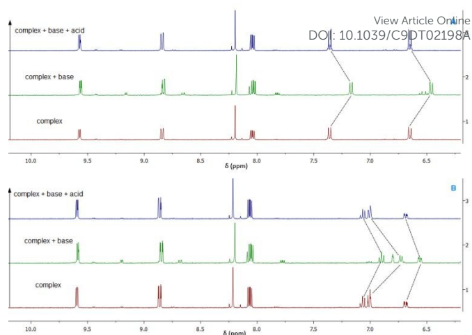
Figure 7. Comparison of 1 H NMR spectra obtained from deuterated methanol solutions containing complex Re4OH (A) and complex Re3OH (B). For each complex, the initial 1 H NMR spectrum is displayed (bottom), along with the addition of base (base), and the sequential addition of acid to reprotonate the phenol ring. The relative changes in the peaks corresponding to the H atoms of the phenol rings are highlighted by the dashed lines.
