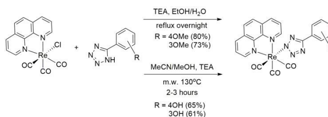
Scheme 2. Reaction scheme for the preparation of the target rhenium(I) complexes.
