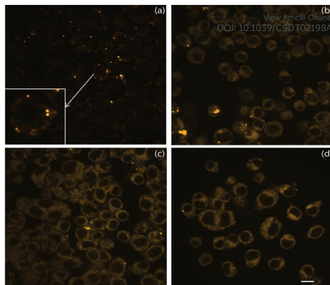
Figure 10. Confocal imaging of RAW264.7 cells incubated with the rhenium complexes for 30 minutes at 10 \mu\text{M} concentration: Re4OH (a), Re3OH (b), Re4OMe (c), and Re3OMe (d). The cells are then fixed using using 4% paraformaldehyde in PBS. Scale bar = 100 \mu\text{m} .
