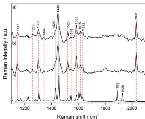
Figure 8. Raman spectra of Re4OH . 351 nm resonance spectra are shown in methanol (a) and methanol with 1 equivalent of KO t Bu (b). Panel c) shows the non-resonant 1064 nm spectrum from a solid state sample.
