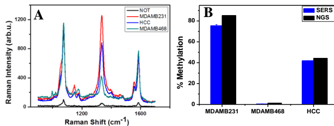
Fig.4. Typical SERS spectra for a panel of cell lines detection (A) and comparison of estimated methylation in three breast cancer cell lines with SERS-LCR assay (B). Error bars represent \pm SD, n=5 .
