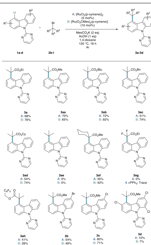
Scheme 2: Ruthenium Catalysed C4-Selective C-H Alkylation of Carbazole Derivatives
