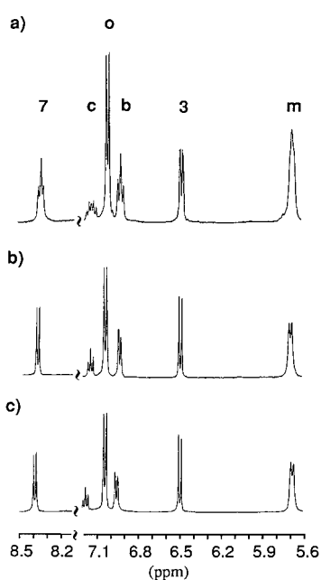
Figure 5. ^1\text{H} NMR at 400 MHz in \text{CD}_2\text{Cl}_2 (aromatic region, selected peaks) of a) the racemate, b) diastereomer (+)\text{-4}^{2+}\cdot 2(+)\text{-BNP}^- and c) diastereomer (-)\text{-4}^{2+}\cdot 2(+)\text{-BNP}^- .
