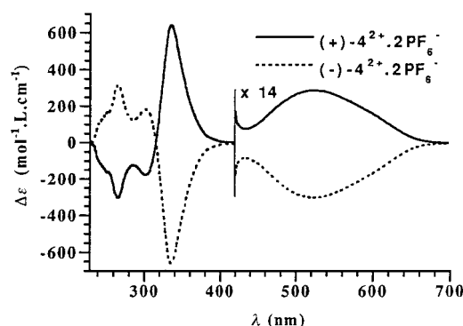
Figure 6. Circular dichroism spectra of both enantiomers of the dicopper(II) trefoil knot (-)\text{-4}^{2+}\cdot 2\text{PF}_6^- (dotted line) and (+)\text{-4}^{2+}\cdot 2\text{PF}_6^- (plain line) in \text{CH}_2\text{Cl}_2 ; these are perfect mirror images.
