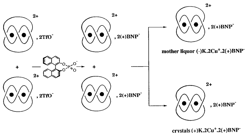
Figure 4. Principle of the resolution of the dicopper(I) molecular trefoil knot 4^{2+} . The chiral auxiliary used is ( S )-(+)-1,1'-binaphthyl-2,2'-diyl phosphate ( \text{BNP}^- ).
