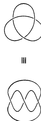
Figure 1. The two topologically equivalent representations of both enantiomers of a trefoil knot.
