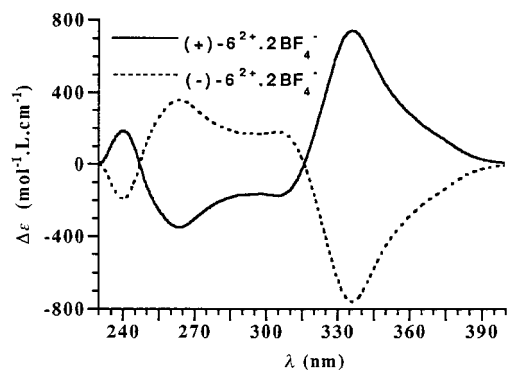
Figure 7. Circular dichroism spectra of both enantiomers of the disilver(I) trefoil knot (−)- 6^{2+} \cdot 2\text{BF}_4^- (dotted line) and (+)- 6^{2+} \cdot 2\text{BF}_4^- (plain line) in \text{CH}_2\text{Cl}_2 .
