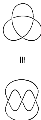
Figure 1. The two topologically equivalent representations of both enantiomers of a trefoil knot.
