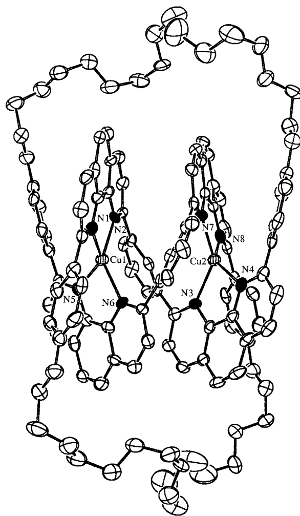
Figure 8. Crystal structure of the dextrorotatory dicopper(I) trefoil knot (+)- 4^{2+} \cdot 2\text{PF}_6^- . ORTEP representation showing the numbering scheme adopted for copper and nitrogen atoms (for the sake of clarity, please note the numbering of the nitrogen atoms is different from the original one reported to Cambridge Crystallographic Data Centre). The solvent molecules, \text{PF}_6^- anions and hydrogen atoms have been omitted and the nitrogen atoms are shown in black.
