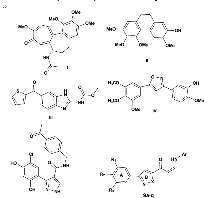
Figure 1A Chemical Structures of some anticancer molecules: Colchicines ( I ), combretastatin A-4 ( II ), nocodazole ( III ), isoxazole derivative ( IV ), pyrazole derivative ( V ) and (Z)-1-(3-aryl-1H-pyrazol-5-yl)-3-(arylamino) prop-2-en-1-one and (Z)-1-(3-arylisoxazol-5-yl)-3-(arylamino) prop-2-en-1-one conjugates ( 9a-q ).
