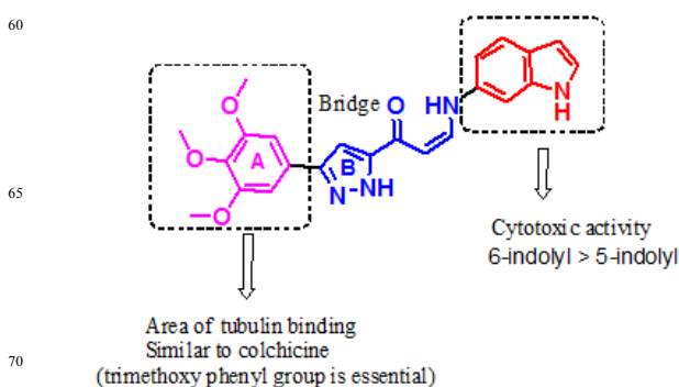
Figure 1B. Structure activity relationship of (Z)-(arylamino)-pyrazolyl/isoxazolyl-2-propenones ( 9a–q ). The compounds that possessing 3,4,5-trimethoxyphenyl as A-ring and indolyl group showed significant anticancer activity. Moreover, 3,4,5-trimethoxyphenyl ring is a hall mark for tubulin binding.
