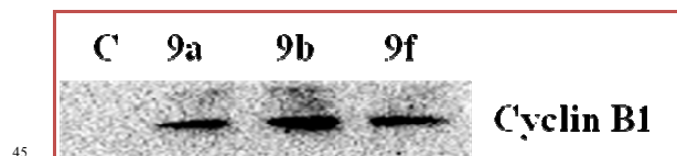
Figure 5. Western blot analysis of Cyclin-B1: Treatment of A549 cells with 2 \mu M concentrations of 9a , 9b and 9f for 24 h resulted an increase in Cyclin B1.
