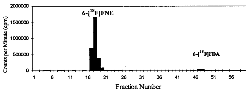
Figure 5. Radiochemical Purity of 6-[ 18 F]FNE Preparation. A sample of the 6-[ 18 F]FNE preparation was loaded onto the ODS HPLC column with the mobile phase flow rate at 1.0 mL/min. Sixty 1-mL fractions were collected into separate tubes by an automatic fraction collector. The collected fractions were then counted for radioactivity.
