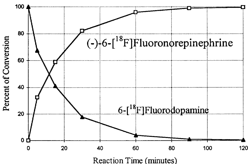
Figure 2. Enzymatic production of 6-[ ^{18}\text{F} ]-fluoronorepinephrine. 1 \mu\text{mole} of 6-[ ^{18}\text{F} ]FDA was incubated in the reaction mixture at 37 ^{\circ}\text{C} with a [\text{D}\beta\text{H}]/[6\text{-[}^{18}\text{F}\text{]FDA}] ratio of 2 units/ \mu\text{mole} . Samples of the reaction mixture were taken at various times for up to 120 minutes. The 6-[ ^{18}\text{F} ]FDA and 6-[ ^{18}\text{F} ]FNE contents in these samples were analyzed by HPLC. The percentages of each of 6-[ ^{18}\text{F} ]FDA and 6-[ ^{18}\text{F} ]FNE relative to the total amount of the two compounds in the reaction mixture samples were plotted as a function of time.
