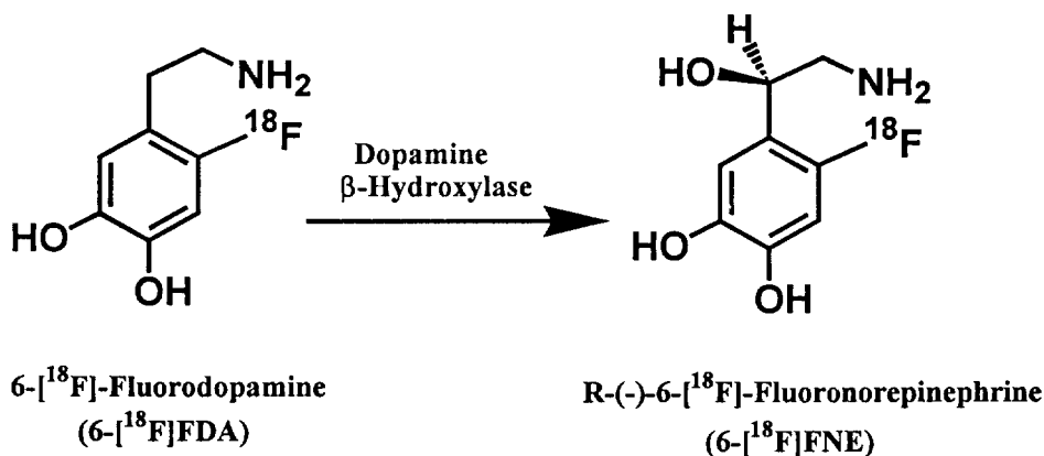
Figure 1. Enzymatic conversion of 6-[ ^{18}\text{F} ]-fluorodopamine to (-)-6-[ ^{18}\text{F} ]-fluoronorepinephrine by dopamine \beta -hydroxylase.
