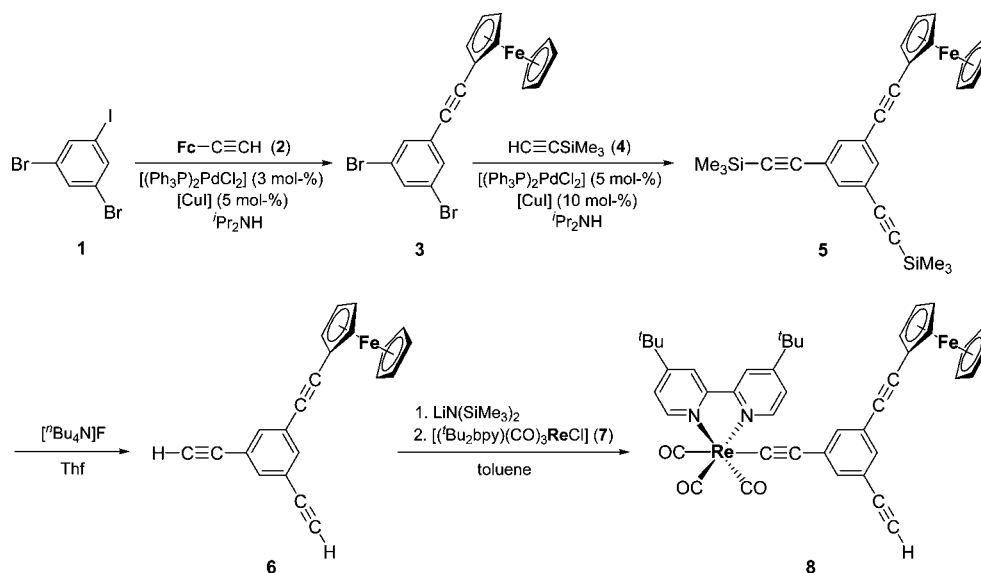
Scheme 1. Synthesis of 8
