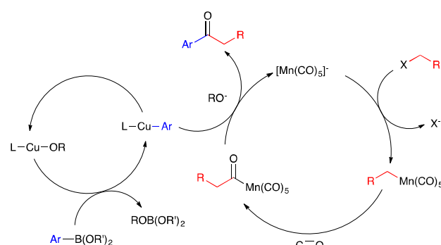
Scheme 1. Bimetallic mechanism for carbonylative Suzuki-Miyaura coupling.
