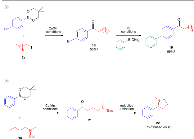
Figure 3. Reaction sequences demonstrating (a) orthogonality of Cu/Mn catalysis and Pd catalysis; (b) relevance of Cu/Mn catalysis to heterocycle synthesis. Cu/Mn conditions: Catalytic conditions: alkyl iodide (0.2 mmol), arylboronic ester (1.5 eq), \text{KOMe} (1.5 eq), (\text{IPr})\text{CuCl} (15 mol%), \text{Na}[\text{Mn}(\text{CO})_5] (7.5 mol%), THF (5 mL), \text{CO} (3 atm), 60^\circ\text{C} , 15 h. Pd conditions: aryl bromide (0.5 mmol), arylboronic acid (2.0 eq), \text{K}_2\text{CO}_3 (2.0 eq), \text{PdCl}_2(\text{PPh}_3)_2 (10 mol%), toluene: \text{H}_2\text{O} (10:1, 5.5 mL), 100^\circ\text{C} , 21 h. Reductive amination conditions: (i) \text{CF}_3\text{CO}_2\text{H} (0.5 mL), \text{CH}_2\text{Cl}_2 (3 mL), 0^\circ\text{C} , 2 h, (ii) \text{NaBH}_4 (4 eq), MeOH (5 mL), 1 h. a Isolated yield. b Yield determined by NMR analysis (1,3,5-trimethoxybenzene internal standard).
