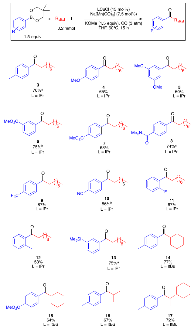
Figure 2. Substrate scope of Cu/Mn-catalyzed carbonylative Suzuki-Miyaura coupling. Yields determined by product isolation unless otherwise indicated. a GC yield (decane internal standard). b From arylboronic acid pinacol ester. c Isolated as 2:1 mixture with N,N -dimethylbenzamide.
