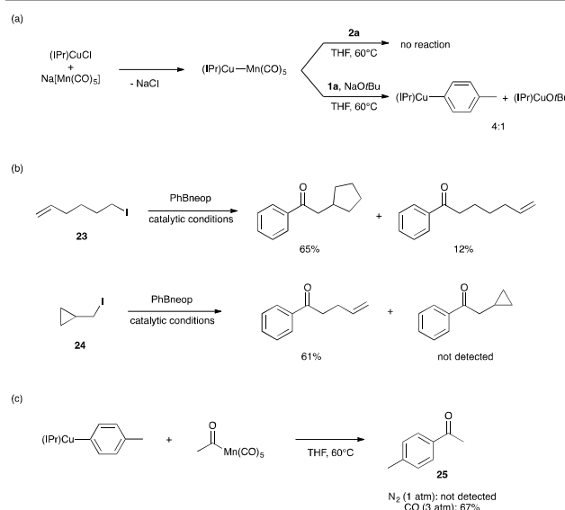
Figure 4. Reactivity studies to probe the catalytic mechanism. Yields determined by NMR analysis (1,3,5-trimethoxybenzene internal standard). Catalytic conditions: alkyl iodide (0.2 mmol), arylboronic ester (1.5 eq), KOMe (1.5 eq), (IPr)CuCl (15 mol%), Na[Mn(CO)_5] (7.5 mol%), THF (5 mL), CO (3 atm), 60°C, 15 h.
