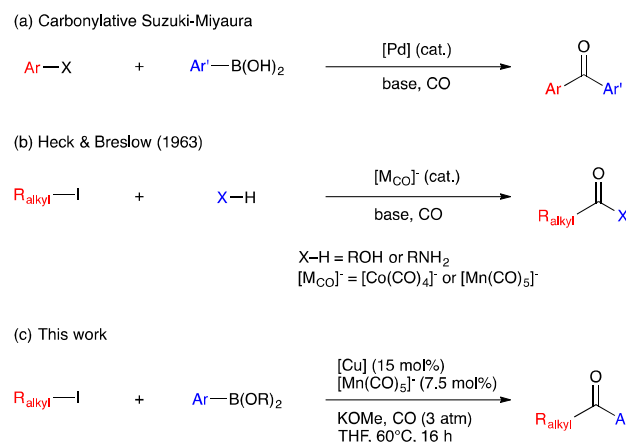
Figure 1. Previous work on (a) Pd-catalyzed Suzuki-Miyaura and (b) base metal-catalyzed heterocarbonylation reactions; (c) this work on base metal-catalyzed carbonylative C-C coupling with alkyl iodides.
