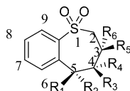
Figure 1. Benzothiepienes.
