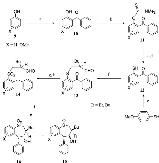
Scheme 2 a
